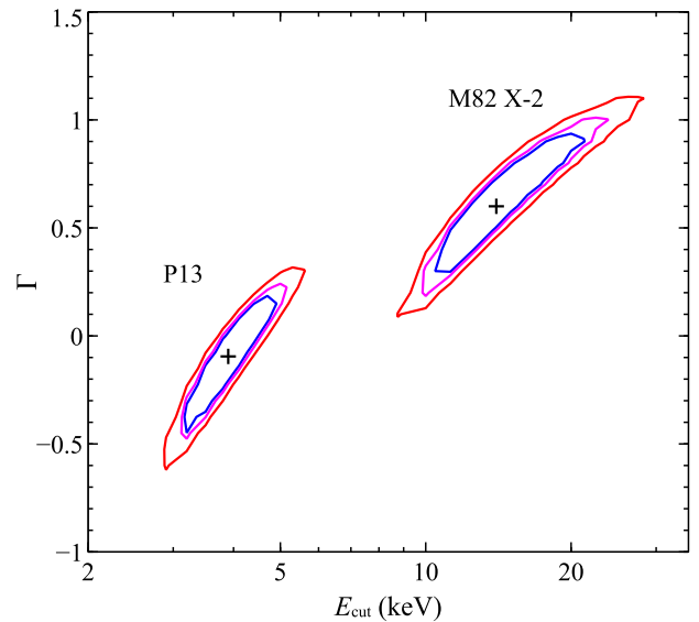
Figure 2. 2D confidence contours for \Gamma and E_{\mathrm{cut}} for the pulsed spectra of P13 and M82 X-2. The 90, 95 and 99 per cent confidence contours for two parameters of interest are shown in blue, magenta and red, respectively.
