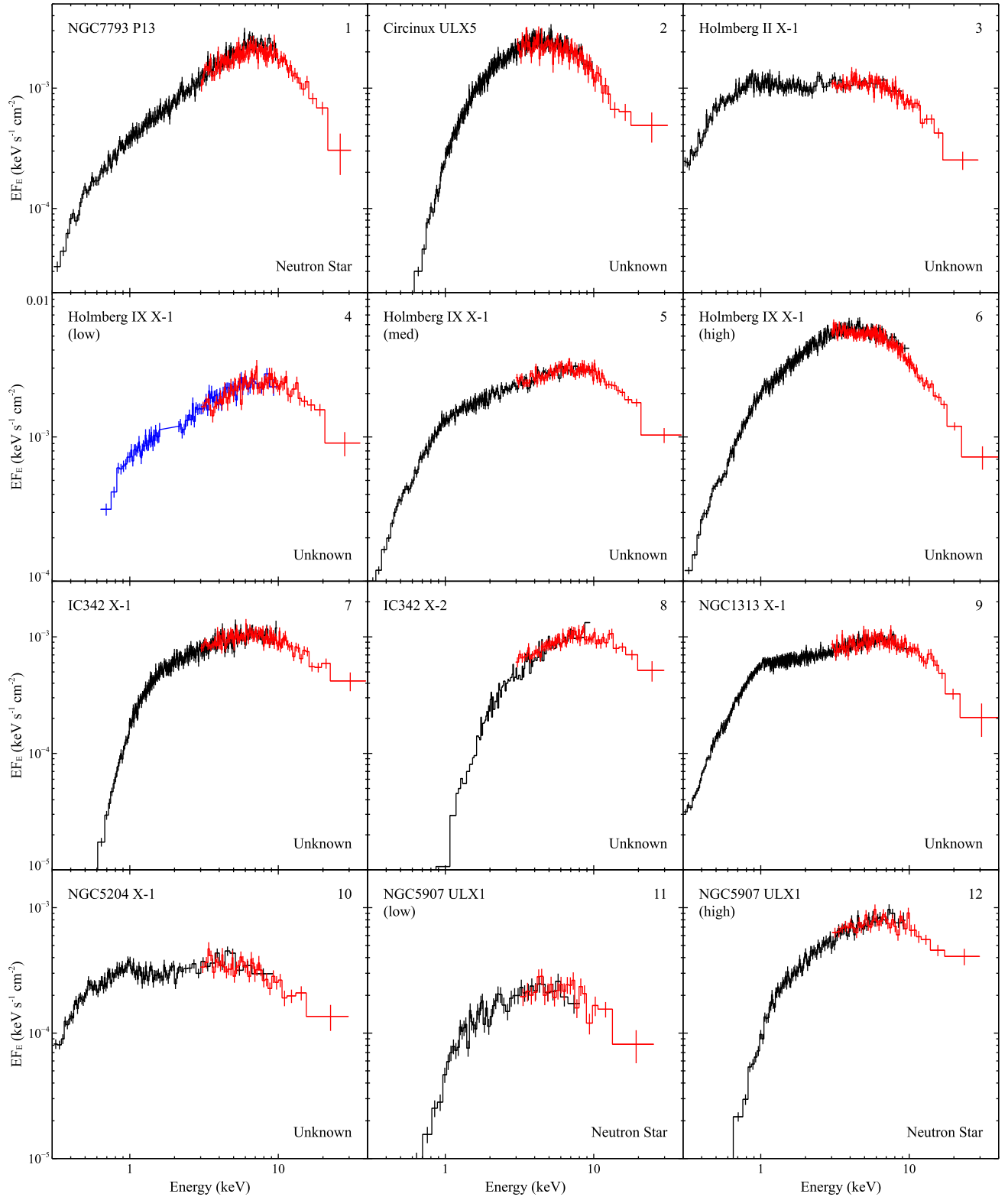
Figure 11. Broad-band spectra of the ULX population with simultaneous coverage in both soft ( XMM-Newton , Suzaku ) and hard ( NuSTAR ) X-rays; as for Fig. 1 (left), the data have been unfolded through a model simply consisting of a constant. Only sources which suffer from negligible source confusion and which are robustly detected out to at least 20 keV are included, and for clarity, only data from the XMM-Newton EPIC-pn (black), NuSTAR FPMA (red) and Suzaku front-illuminated XIS (blue) detectors are shown (the only exception is NGC 5907 ULX, where for NuSTAR we show the combined FPMA+FPMB data owing to the lower S/N in this case). The sample includes P13 (panel 1; this work), Circinus ULX5 (panel 2; adapted from Walton et al. 2013), Holmberg II X-1 (panel 3; adapted from Walton et al. 2015b), Holmberg IX X-1 (panels 4–6; adapted from Walton et al. 2017), IC 342 X-1 and X-2 (panels 7 and 8, respectively; adapted from Rana et al. 2015), NGC 1313 X-1 (panel 9; adapted from Bachetti et al. 2013), NGC 5204 X-1 (panel 10; adapted from Mukherjee et al. 2015) and NGC 5907 ULX (panels 11–12; adapted from Fürst et al. 2017).
