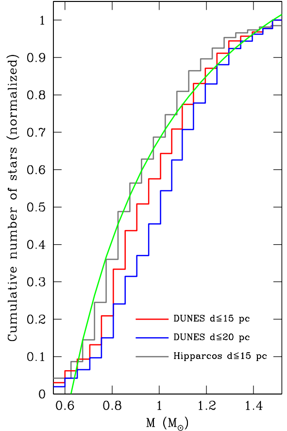
Fig. 2. Cumulative distributions (normalized) for the DUNES samples with d \leq 15 pc (105 stars, red) and d \leq 20 pc (177 stars, blue) and the FGK stars in the HIPPARCOS catalogue with d \leq 15 pc (154 stars, grey), all plotted against stellar mass. A Salpeter law with exponent -2.35 has been normalized to the distributions. See text for details.
