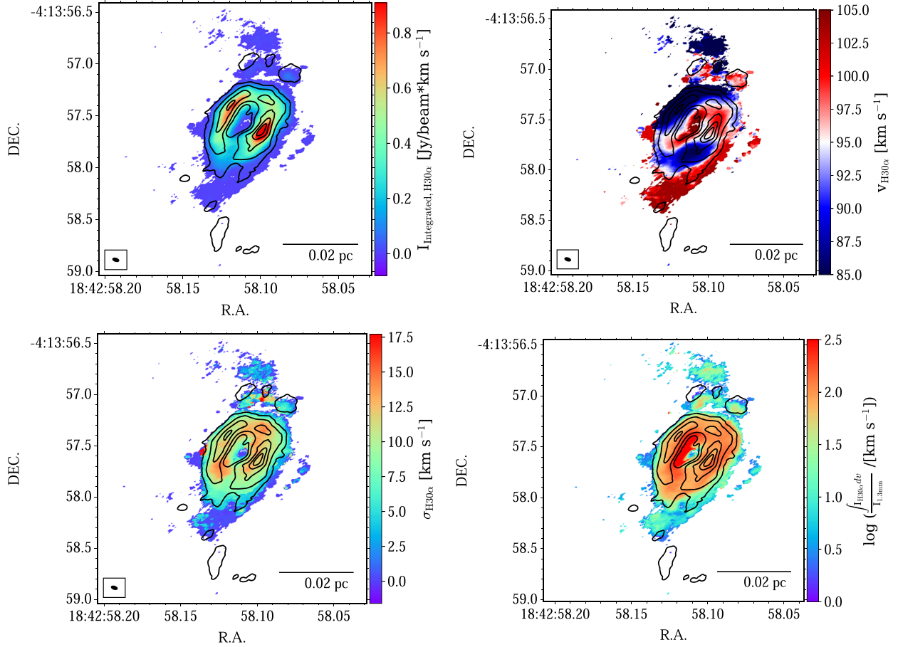
Figure 10. (a) Top left: H30 \alpha moment zero map, only considering pixels with integrated intensity above 5\sigma of the spectral rms measured over emission free velocity channels in the averaged velocity spectrum (note, 1\sigma \simeq 0.8 \text{ mJy beam}^{-1} ). The black contours show the 1.3 mm continuum emission (0.5, 1, 1.5, 2, 2.5, 3, 3.5, 4, 4.5, 5, 5.5, 6 Jy arcsec ^{-2} ). (b) Top right: as (a), but now showing the H30 \alpha moment one map, i.e., averaged line-of-sight velocity. (c) Bottom left: as (a), but now showing the H30 \alpha moment two map, i.e., the 1D velocity dispersion along the line of sight of the H30 \alpha emission. (d) Bottom right: as (a), but now showing the ratio between the integrated intensity of H30 \alpha and the continuum intensity.
