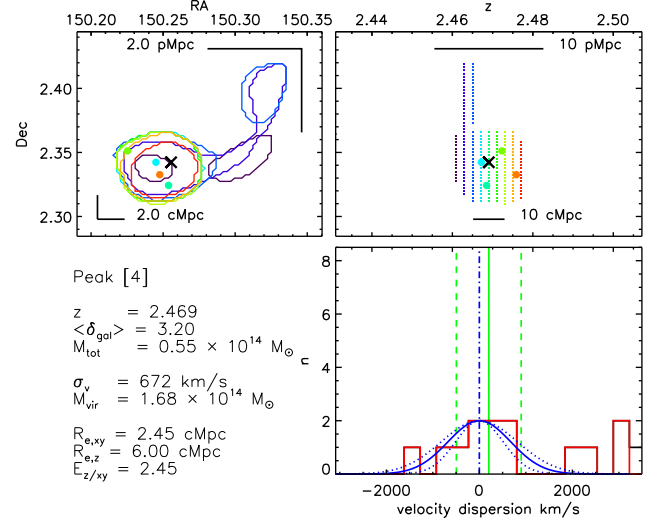
Fig. B.4. As in Fig. B.1, but for Peak [4], “Selene”.
