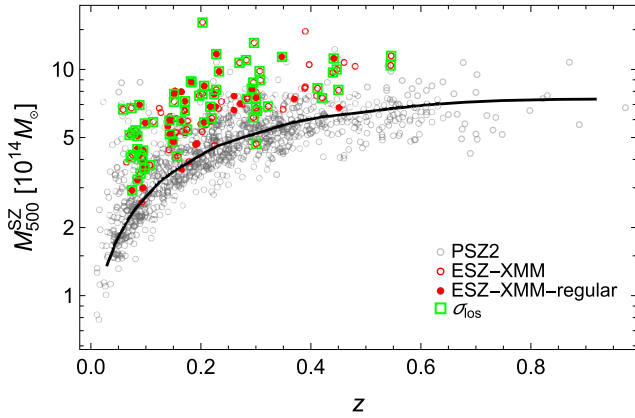
Figure 1. Sample. Shown is the distribution in the M_{500}^{\text{SZ}}-z plane of the ESZ-XMM clusters (red circles). The X-ray morphologically regular clusters are marked as red discs. The 1094 PSZ2 clusters with known-redshift counterparts are shown as grey circles. The ESZ-XMM clusters with measured galaxy velocity dispersion are marked with a green square. The solid line indicates the average 80 per cent survey completeness limit for PSZ2. The mass M_{500}^{\text{SZ}} is based on a SZ proxy. For the five ESZ-XMM clusters with no counterpart in the PSZ2 catalog, we plot the hydrostatic mass. M_{500}^{\text{SZ}} is computed within r_{500} , the radius within which the average cluster matter density is 500 times the critical density of the universe at the cluster redshift.
