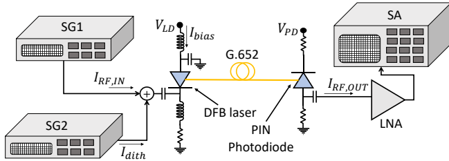
Fig. 2. Experimental setup utilized for the characterization of the optimum frequency and amplitude of the dithering tone to suppress the Rayleigh Backscattering. Signal generator (SG) 1 is used for emulating the RFI tones, while SG2 is used for generating the dithering tone. The harmonics are then measured with a Spectrum Analyzer (SA).
