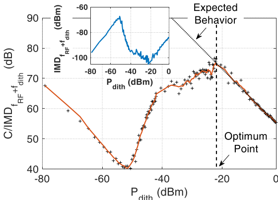
Fig. 6. C/IMD_{f_{RF}+f_{dith}} vs. P_{dith} with f_{dith} = 8 KHz and P_{RF,IN} = -33 dBm. The ideal behavior is modelled by taking a_2 = 0.35 .
