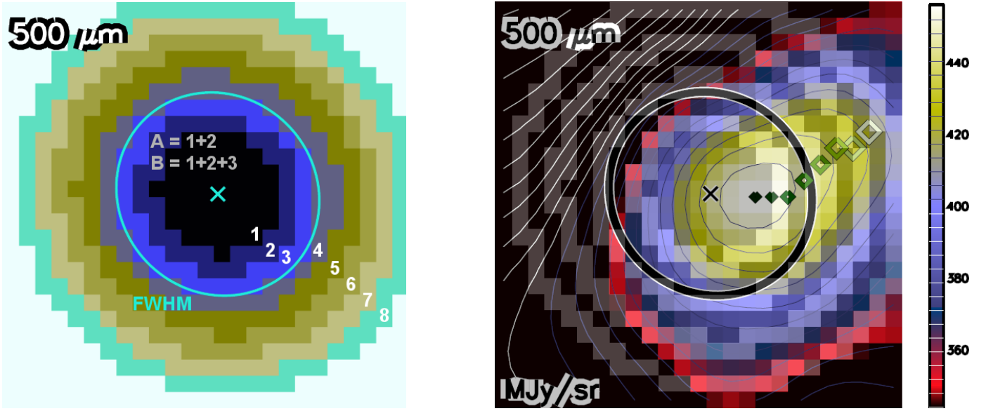
Fig. B.2. Left: examples of annular masks created inside and outside of the FWHM ellipse of each core at each wavelength. The example mask image shown here is at 500\ \mu\text{m} and belongs to the prestellar core of Fig. B.1. Inside out, the division of the masks along the core radius is the following, considering the FWHM ellipse as 100%: region 1: <60% interior of the FWHM radius, region 2: 60–80%, 3: 80–100%, 4: 100–120%, 5: 120–140%, 6: 140–160%, 7: 160–180%, 8: 180–200%. Region A: <80% (regions 1+2), B: <100% (1+2+3). Right: the first maximum (i.e., the highest intensity pixel) in each mask is shown by a green-shaded diamond in the example image. The panel size, marked source center, and FWHM sizes are the same for each pair of mask image and observed image.
