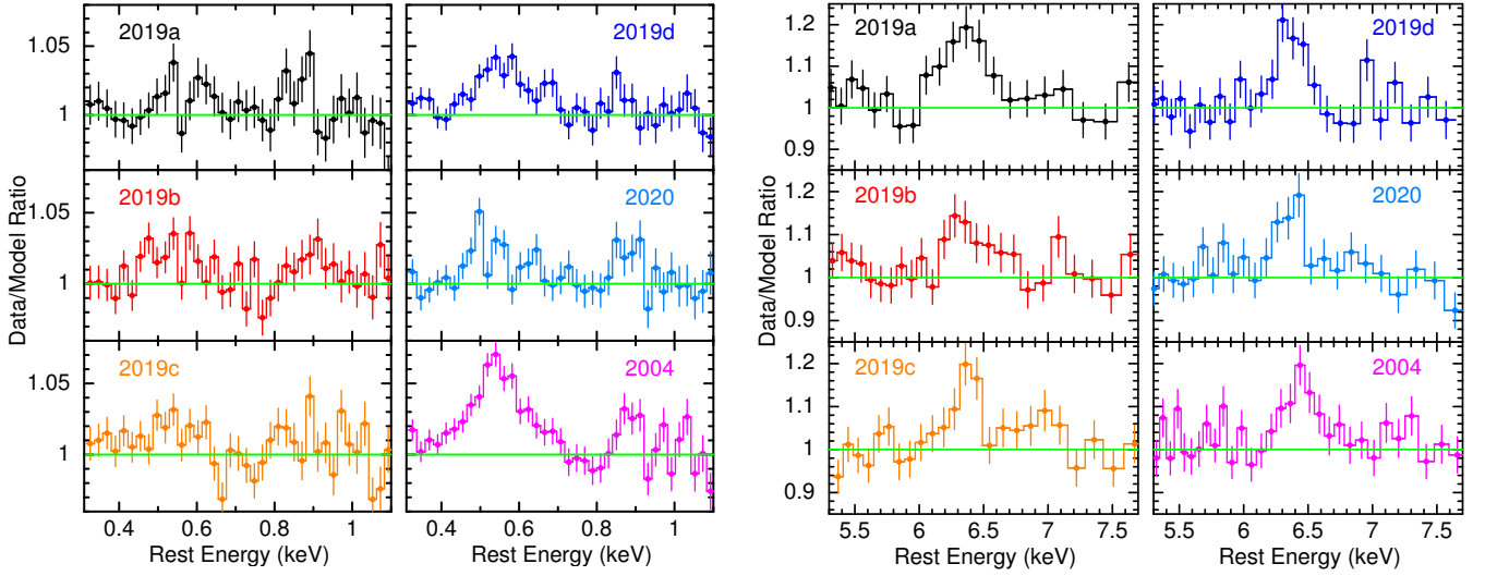
Fig. A.3. Six left panels: EPIC-pn ratio residuals of all six spectra between 0.3–1.1 keV, compared to the two component continuum model as described in the main text. Significant excess residuals are seen over the 0.5–0.6 keV O VII line region, in particular towards the 2004, 2019d, and 2020 pn spectra, where the thin filter was in place. The excess emission can be fitted with a Gaussian profile, with line fluxes as reported in Table A.1. As per the RGS analysis, the pn data show a similar trend between the line flux and the continuum, whereby the strongest line emission is found in the brightest (2004) observation and the weakest line flux is found in the two faintest (2019a, 2020) observations. Six right panels: Equivalent data/model ratio plots showing all six pn spectra over the iron K band, where the iron line emission is less variable.
