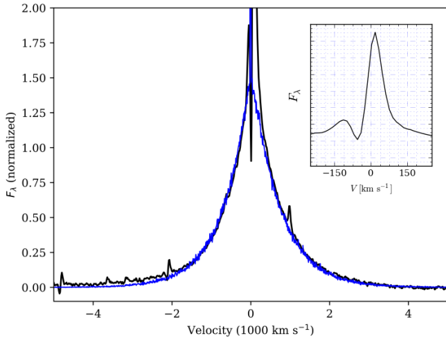
Fig. 12. H\alpha line profile observed in the +46 d Keck DEIMOS spectrum of SN 2015da along with a fit to the line profile from electron scattering. The line profile below \pm 200 \text{ km s}^{-1} , in the model from un-scattered photons, is affected by the resonance line scattering in the H\alpha transition and was not modeled.
