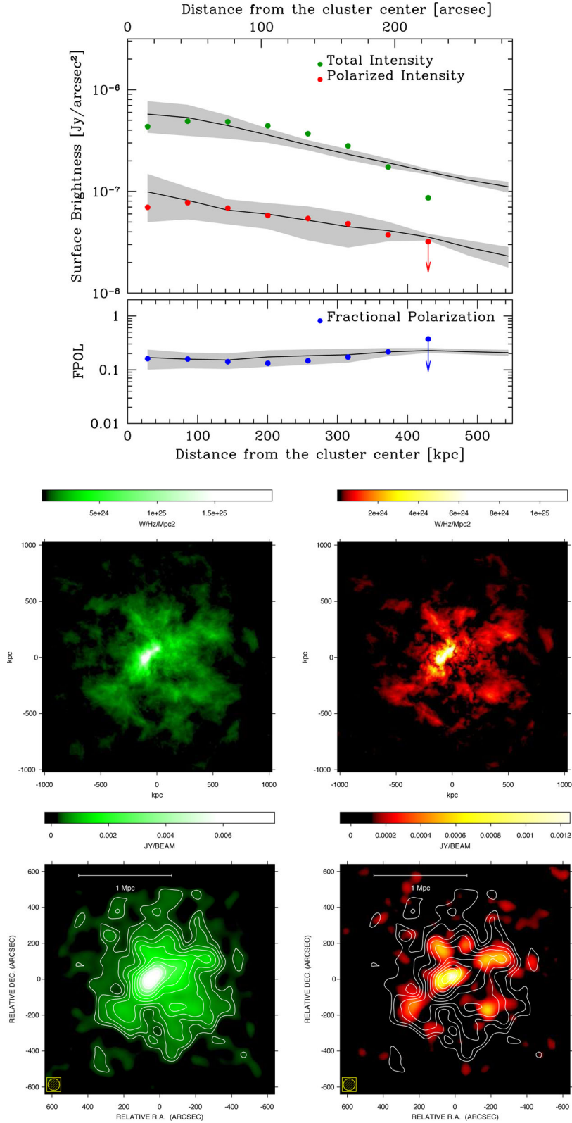
Figure 19. Top panels: azimuthally averaged radio-halo brightness profiles of the total intensity I (green dots), polarized intensity P (red dots), and FPOL (blue dots). The profiles have been calculated in concentric annuli, as shown in Fig. 18. The continuum line and the shade region in the top panels describe the mean and the sigma of a set of simulations with different random seeds performed with a magnetic field model which is able to describe the data quite well. This model is a Kolmogorov magnetic field power spectrum with a central magnetic field strength of 0.5 \mu\text{G} which fluctuates in a range of scales from a few h_{70}^{-1} \text{ kpc} up to \sim 1 h_{70}^{-1} \text{ Mpc} and decreases with the gas density as B(r) \propto n_e(r)^{0.5} . Middle panels: example of a simulated radio halo at full resolution obtained with the above magnetic field model. Left and right panels refer to the total intensity and polarized surface brightness images, respectively. Bottom panels: the images show as the simulated radio halo would appear when observed at the same resolution and sensitivity of A523. The white contour levels refer to the total intensity image at 65 arcsec resolution. Contour levels start at 0.3 \text{ mJy beam}^{-1} and increase by a factor of \sqrt{2} .
