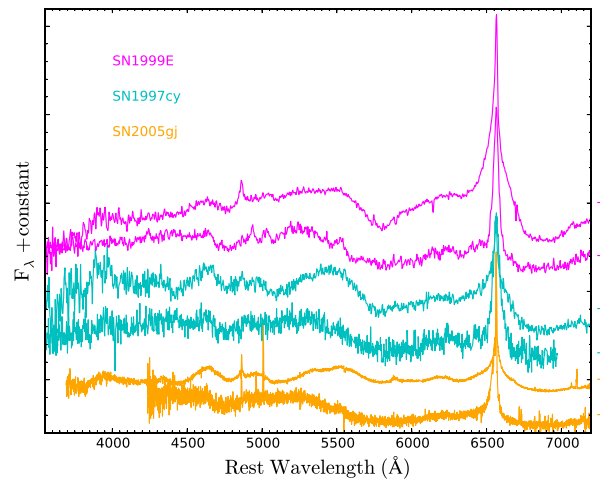
Figure 8. Late time (>400 d) spectra of SNe 1997cy, 1999E and 2005gj.
