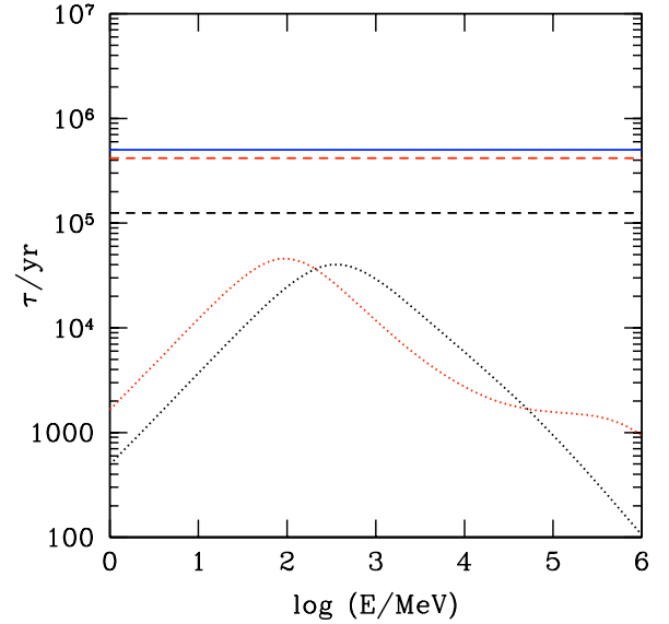
Fig. 1. Residence times of CR protons (dashed) and electrons (dotted) in the CND of NGC 1068 as a function of the particle's energy. Red lines: n_H = 120 \text{ cm}^{-3} , B_{\text{ISM}} = 100 \mu\text{G} , L_{\text{AGN}} = 2.1 \times 10^{45} \text{ erg s}^{-1} , U_{\text{rad}} = 3.7 \times 10^4 \text{ eV cm}^{-3} , R_{\text{shock}} = 100 \text{ pc} , and v_{\text{shock}} = 200 \text{ km s}^{-1} ; black lines: n_H = 400 \text{ cm}^{-3} , B_{\text{ISM}} = 350 \mu\text{G} , L_{\text{AGN}} = 4.2 \times 10^{44} \text{ erg s}^{-1} , U_{\text{rad}} = 7.3 \times 10^3 \text{ eV cm}^{-3} , R_{\text{shock}} = 100 \text{ pc} , and v_{\text{shock}} = 200 \text{ km s}^{-1} . The solid blue line indicates the timescale of the AGN-driven molecular outflow.
