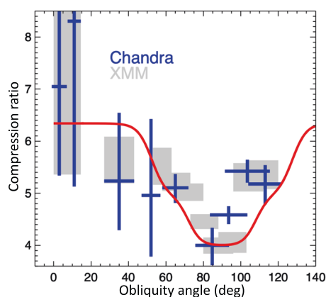
Fig. 6 | Modulation of the shock compressibility in a non-uniform magnetic field. Same as Fig. 3, with the solid curve marking the profile expected for \xi_p = 12\% , \xi_s = 5\% and \xi_B = 6\% , but including a gradient of the magnetic field strength, lying in the plane of the sky at \theta = 90^\circ . Source data are provided as a Source Data file.
