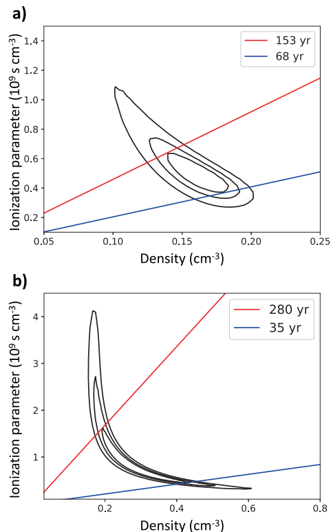
Fig. 4 | Ionization parameter and post-shock density. 68%, 90%, and 99% confidence contour levels of the ISM density and ionization parameter derived from the Chandra spectra of region 0 (a) and region 5 (b). Red and blue lines mark isochrones after the interaction with the shock front.
