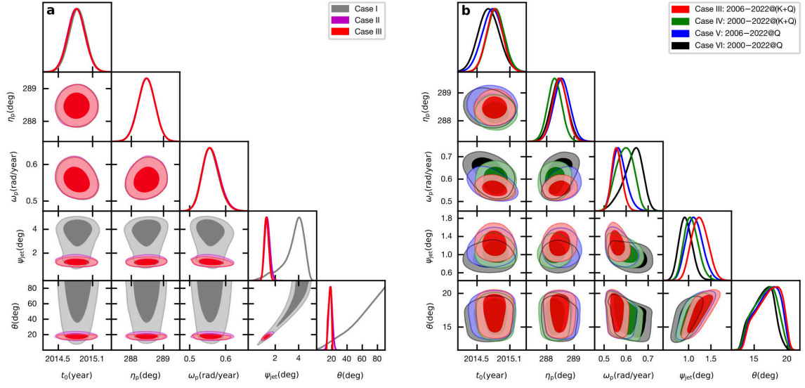
Extended Data Figure 3: Posterior distributions of precession model parameters in different cases. (a): comparison among Case I–III with different constraints. (b): comparison among Case III–VI with different data sets. The detailed information for each case is described in Extended Data Table 4 and Methods. The contours correspond to the 68% and 95% confidence levels.
