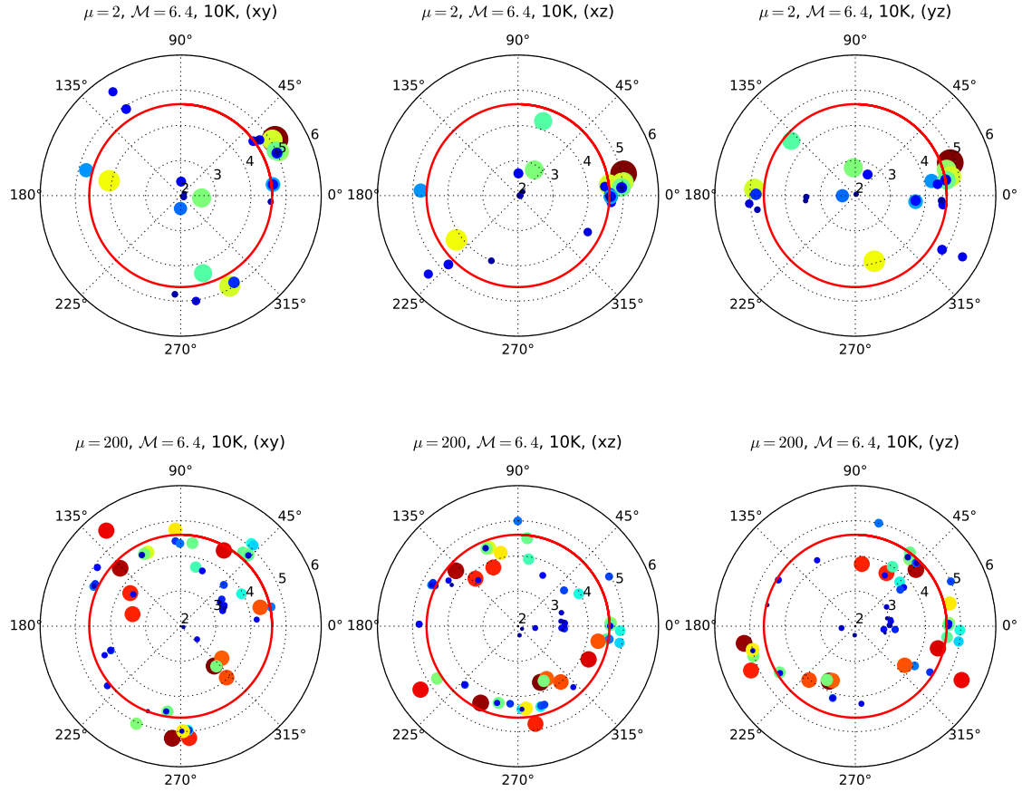
Fig. B.2. Projected sink particle distribution centered around the most massive sink particles at an SFE of 15% for simulations (3) ( M \sim 6.4 , T = 10\text{K} ). The radial direction shows the distance in au in logarithmic scale. The red circle represents the size of the region that we post-processed with CASA to produce the ALMA synthetic observations.
