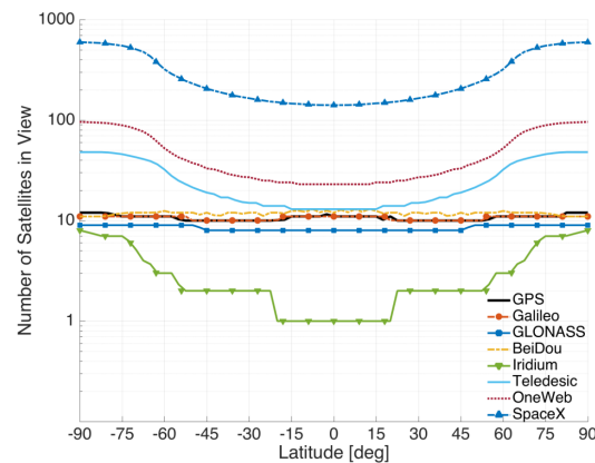
Fig. 2 Number of satellites in view vs. latitude (graphic from: https://pdfs.semanticscholar.org/487e/24483f22b43d57da78772dac9d20a948ec23.pdf )
