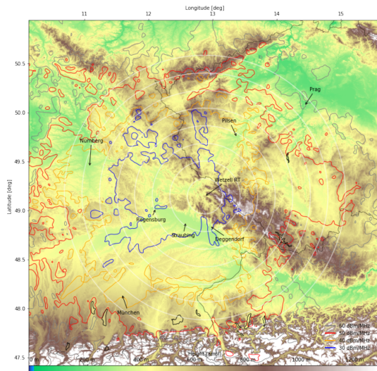
Fig. 1 Compatibility study for Wettzell site: coordination zone for 5G at 3.4 GHz (blue 30dBm/MHz, red 50dBm/MHz). White circles mark distances to the RAS station in steps of 20 km.
