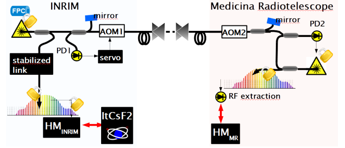
Fig. 2. The setup of our experiment. A fiber laser is frequency-locked to a high-finesse Fabry-Pérot cavity (FPC) and used as a transfer laser. Its frequency is measured against HM_{INRIM} using a fiber optical frequency comb; HM_{INRIM} is constantly measured by the primary frequency standard ItCsF2. The transfer laser is sent to Medicina Radiotelescope (MR) via a phase-stabilized optical link and here regenerated by phase-locking a diode laser to it. The regenerated radiation is used as a reference to stabilize an optical comb; the 40th harmonic of the repetition rate is extracted, divided by 100 and compared to HM_{MR} . AOM: acousto-optic modulators; PD: photodiodes; triangles represent bidirectional Erbium-Doped Fiber Amplifiers
