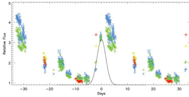
Figure 3. NEOWISE multi-color ( W1, W2, W3, W4) light curve of G107, folded by the 34.6 d period, and normalized to minimum brightness. Zero represents the date of the maser flare peak. Large crosses mark IRAC flux ratios, normalized to the low state. The Gaussian fit to the methanol maser light curve (Fujisawa et al. 2014) is shown for comparison. The apparent jumps at phase of \sim 4 d are due to long-term brightening. See online paper for color figure.
