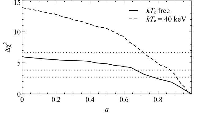
Figure 6. The \Delta\chi^2 confidence contours for the spin parameter from our preferred model for the broadband data of IRAS 00521–7054 (Model 2, see Section 3.2). We show contours computed with the electron temperature free to vary (solid line) and assuming a temperature of kT_e = 40 keV (dashed line). The horizontal dotted lines represent the 90, 95 and 99% confidence levels for a single parameter of interest.
