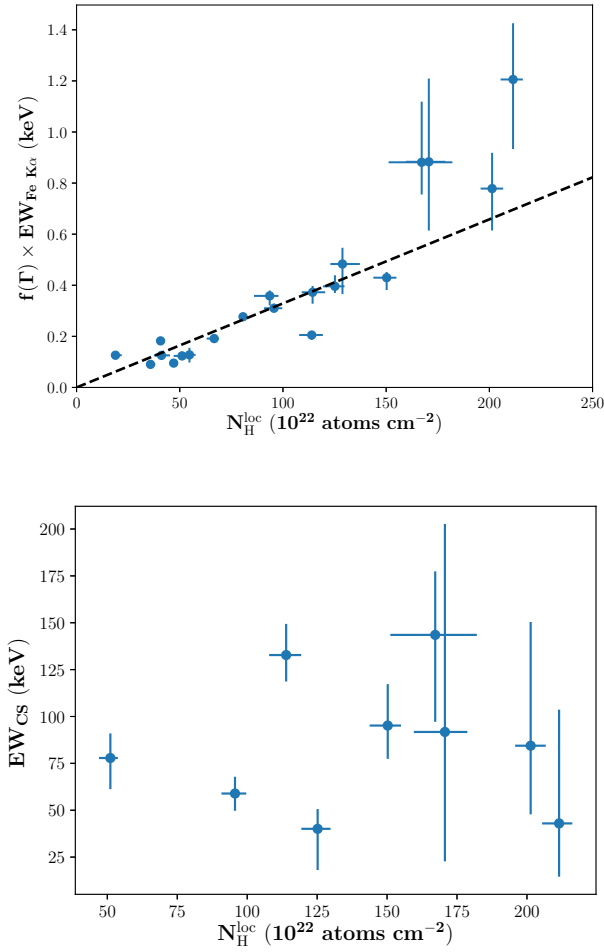
Figure 5. The upper (bottom) panel shows equivalent widths of Fe K \alpha lines (CSs) as a function of the local absorption column N_{\text{H}}^{\text{loc}} . The black dashed line represents the theoretical estimation ( \text{EW}_{\text{Fe K}\alpha}(\text{eV}) \approx 3 \times 10^{-22} N_{\text{H}} ) assuming a spherical shell of gas surrounding a point source of continuum radiation (Kallman et al. 2004).
