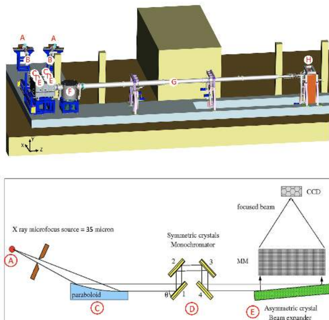
Fig. 2. Schematic of the BEaTriX facility: two-beamline layout and coordinate system, (top) and optical design for the 4.51 keV beamline (bottom). The optical components enable collimation, spectral filtering, and expansion of an X-ray beam.
