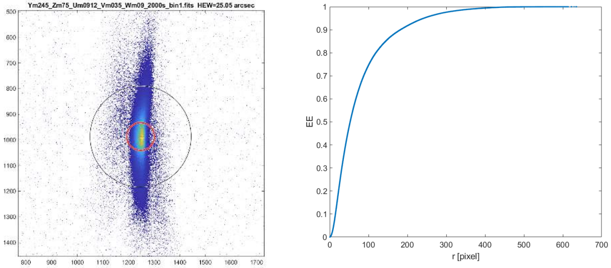
Fig. 7. Acquired image of MM-0042. Left: pixel size is 13.5 \mu\text{m} , and the two circles correspond to the HEW and the diameter enclosing 90% of the collected photons (W90). Right: measured encircled energy (EE; the radial integration of the PSF) function of the MM-0042, used to retrieve the HEW and the W90 of the module.
