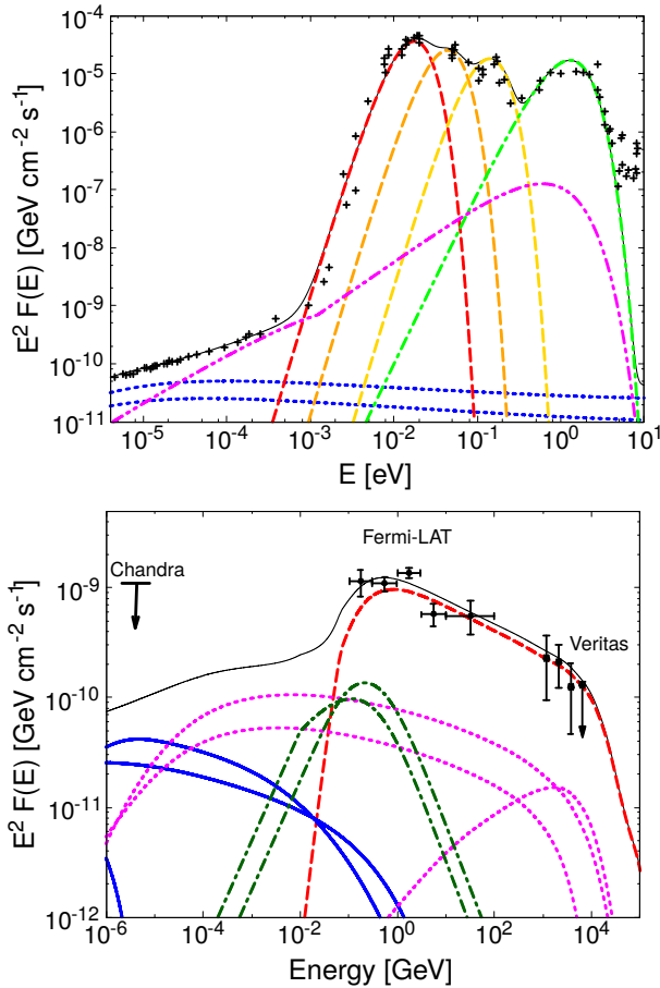
Figure 6. Multiwavelength spectrum of M82. The line style is the same of figure 5. The HE gamma-ray observation are taken from the Fermi-LAT observation discussed in Acero et al. (2015) , whereas VHE data come from Veritas and are published in Acciari et al. (2009) . The X-ray point is a Chandra (see Strickland & Heckman 2007 ) we have taken as upper limit because of possible contamination from undetected point-like sources (e.g. XRBs) and thermal plasma.
