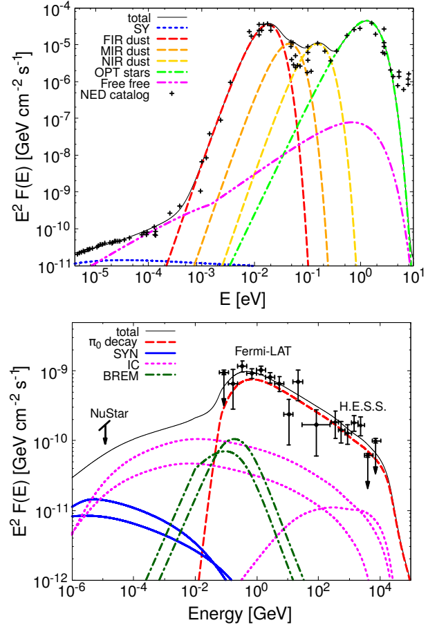
Figure 5. Multifrequency spectrum of NGC253. Upper panel shows the low energy spectrum with relative components: thermal dust DBBs (red, orange and yellow dashed), optical star BB (green dot-dashed), thermal free-free (magenta dot-dot-dashed) and SYN (blue dotted). Lower panel shows the high energy spectral components: \pi_0 (red dashed), IC (magenta dotted), BREM (green dot-dashed) and SYN (blue dashed). Together with the photons we show the single flavor neutrino flux (thin gold dashed). The data (black points) are observed by Fermi-LAT and HESS and presented in Abdalla et al. (2018) for the HE and VHE domain, whereas the hard X-ray upper limit is taken from Wik et al. (2014).
