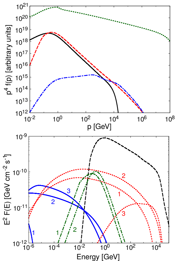
Figure 3. Particle and photon spectra in Model B. The line style is the same as in Figure 2.
