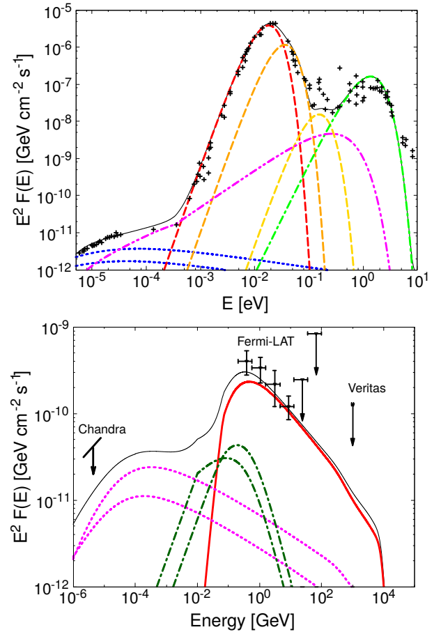
Figure 7. Multiwavelength spectrum of Arp220. The line style is the same of figure 5. Gamma-ray data are taken from Peng et al. (2016) , whereas the X-ray point (which again we take as upper limit for our diffuse flux taking into account possible contamination from pointlike sources and thermal plasma) has been taken from Paggi et al. (2017) .
