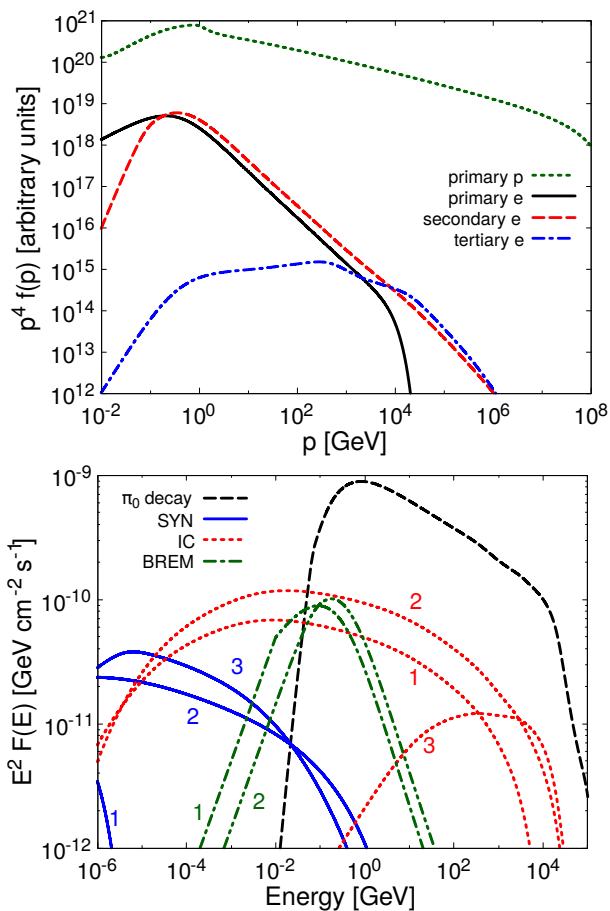
Figure 2. Particle and photon spectra in Model A. The upper panel shows primary protons (green dashed), primary electrons (black thick line), secondary electrons (red dashed line) and tertiary electrons (blue dot-dashed line). The lower panel shows the high energy spectral components of \pi_0 decay (black dashed line), inverse Compton (red dotted line), synchrotron (blue thick line) and bremsstrahlung (green dot-dashed line). The relative contributions of the different electron populations are separated in primaries (1), secondaries (2) and tertiaries (3).
