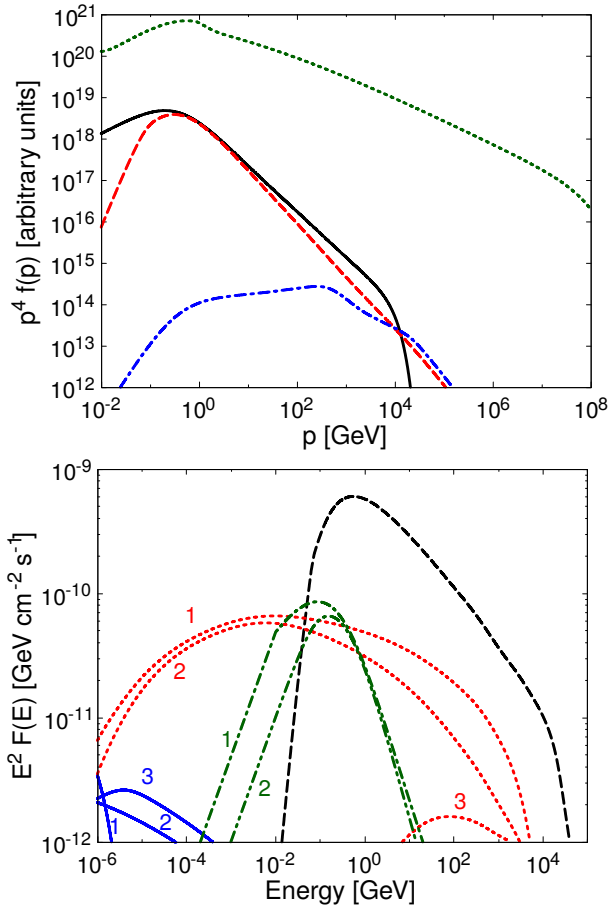
Figure 4. Particle and photon spectra in Model C. The line style is the same as in Figure 2.
