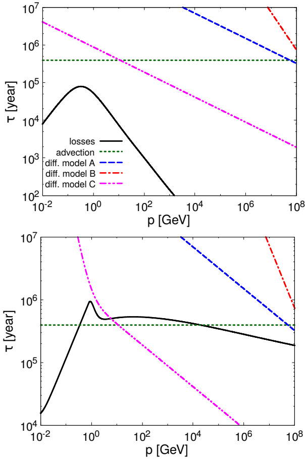
Figure 1. Energy dependence of the characteristic timescales (expressed in years) of cosmic ray electrons (upper panel) and protons (lower panel) for the parameters of our reference case. Black thick lines represent energy losses, green dotted lines show the advection timescales. The timescales of diffusion are represented by blue dashed lines in the case of Kolmogorov, red dot-dashed in the case of Bohm and magenta dot-dot-dashed in the MW-like case.
