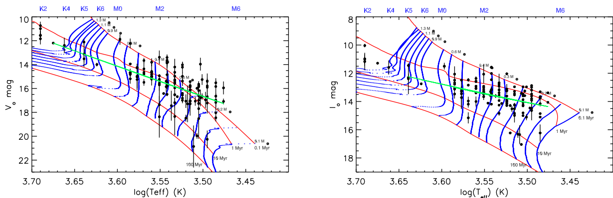
Figure 13. T_{\text{eff}} - V_0 (left panel) and T_{\text{eff}} - I_0 (right panel) diagrams of the ONC members under analysis for which the extinction is known. The black bullets represent the mean magnitudes (average magnitudes over a 5-yr long time series), the vertical bars their range of variation (brightest minus faintest magnitudes). Red solid lines and blue dotted lines represent theoretical isochrones and mass tracks, respectively, from Siess et al. (2000).
