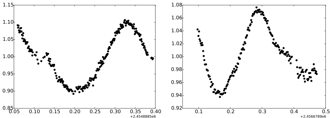
Figure 3: Example lightcurves of (506) Marion. For references to the observations, see text.
