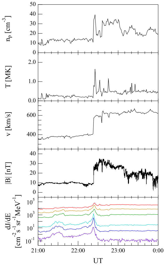
Figure 1. Time history of solar wind plasma parameters and energetic particle fluxes as recorded by STEREO B s/c between 21:00 UT and 24:00 UT on 2011 October 3. From top to bottom: proton density n_p and temperature T , bulk speed v , magnetic field magnitude, and the proton differential fluxes for a selected number of energy channels ( E \sim 0.53, 1.05, 2.10, 4.74, 6.93 , and 10.95 MeV from top to bottom).
