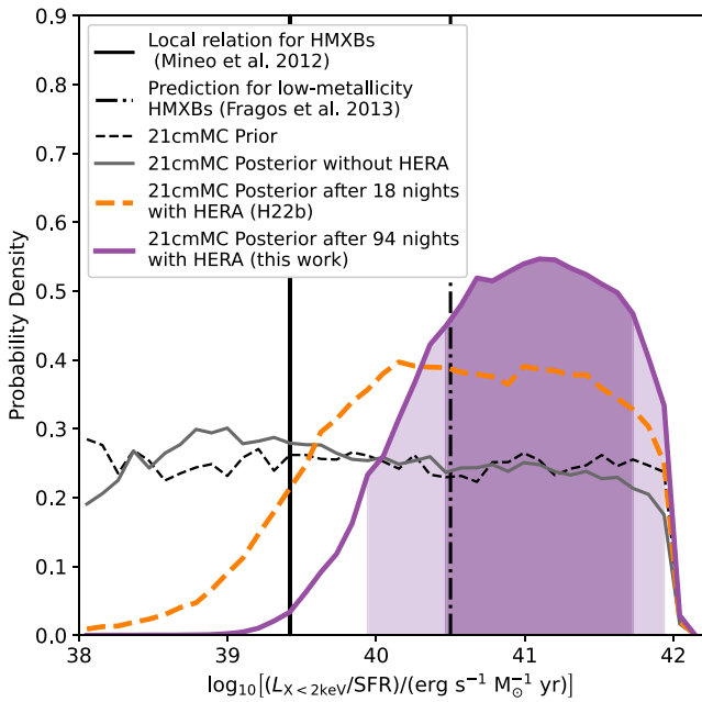
Figure 28. Here we show how our marginalized 21cmMC posterior PDF of the ratio of soft X-ray luminosity to SFR, L_{X<2 \text{ keV}}/\text{SFR} , tightens with a full season of HERA data. The shaded regions show the 68% and 95% credible intervals of the posterior. Probability densities are plotted per logarithmic interval. Our results are consistent with theoretical expectations for X-rays produced during the cosmic dawn by a population of low-metallicity high-mass X-ray binaries (HMXBs; Fragos et al. 2013), likely a more representative model of the first galaxies (dashed-dotted black vertical line). Compared to H22b (orange dashed line), our result’s 99% credible interval excludes models where the local relation for X-ray efficiency (solid black vertical line; Mineo et al. 2012) continues to hold at high redshift.
