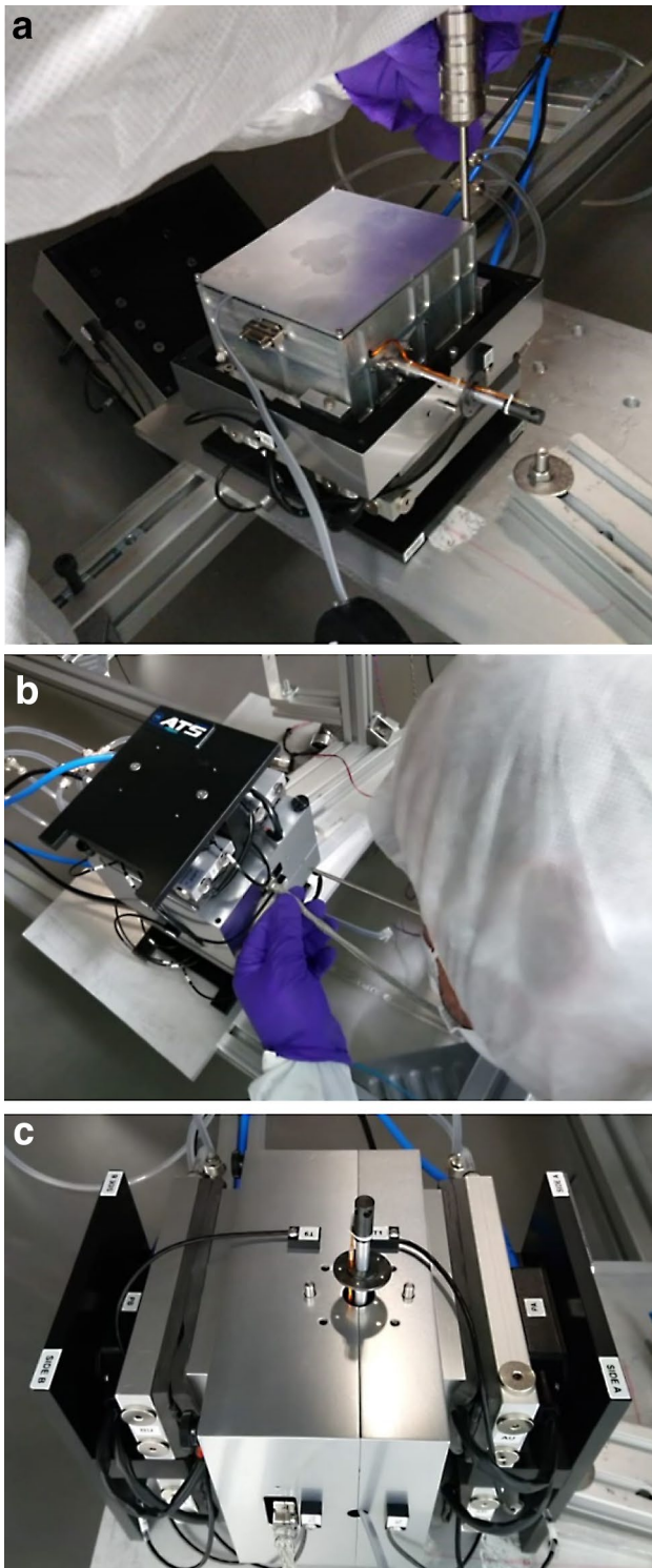
Fig. 8 a MicroMED being fixed inside one of the shells of the ATS “Glove-Box”. b MicroMED installation inside ATS at OAC. c “Glove-Box” closed embracing MicroMED
