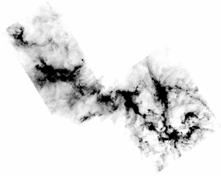
Fig. 1. The column density map of the Perseus complex; black areas are denser. The molecular hydrogen column density runs from 2.5 \cdot 10^{20} \text{ cm}^{-2} up to 1.4 \cdot 10^{23} \text{ cm}^{-2} .
