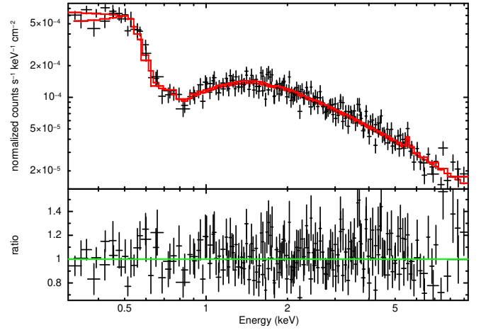
Fig. D.8. Spectrum and ratio of Obs. 11. The red line is the best fit.
