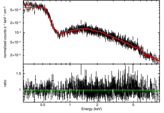
Fig. D.6. Spectrum and ratio of Obs. 8+9. The red line is the best fit.
