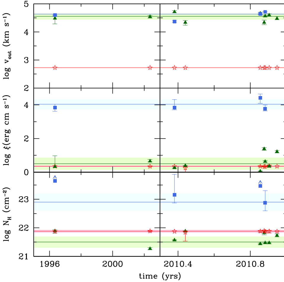
Fig. 4. Time dependence of the outflow velocity v_{\text{out}} (top), ionization parameter \xi (middle), and column density N_{\text{H}} (bottom). For each panel we show the values of Abs. 1 (red stars), Abs. 2 (green triangles), and Abs. 3 (blue squares). Lower limits on N_{\text{H}} were marked with an arrow. Horizontal lines with shaded bands represent the median values and the corresponding median absolute deviations.
