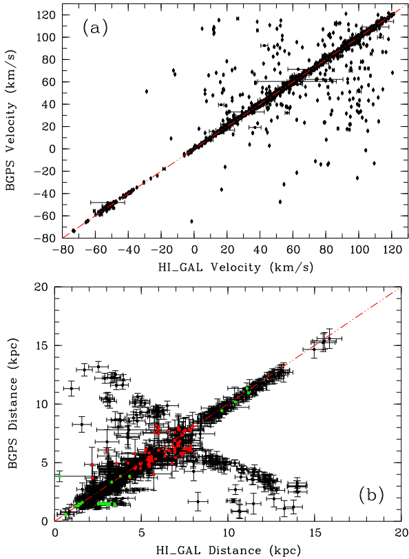
Fig. 11. (a) Velocity (2285 sources) and (b) distance (2050 sources) comparison between paired BGPS and Hi-GAL sources. The red dashed line is the y = x line. Same color coding as in Fig. 10.
