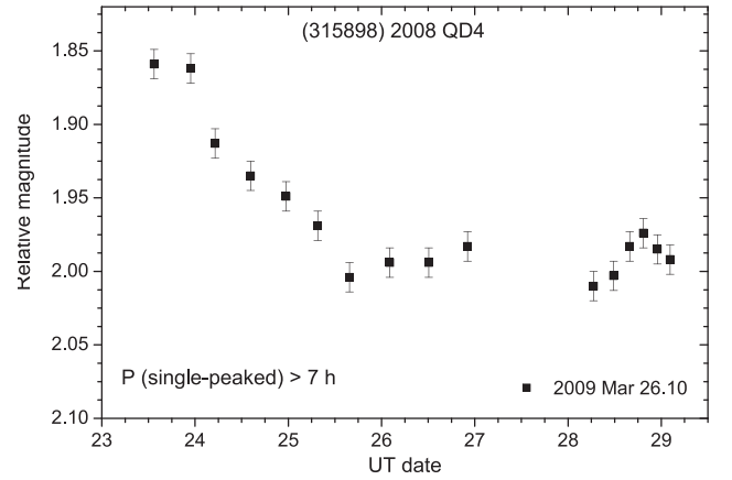
Figure 12. Light curve of (315898) 2008 QD4.
