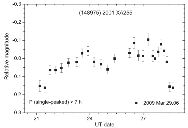
Figure 7. Light curve of (148975) 2001 XA255.
