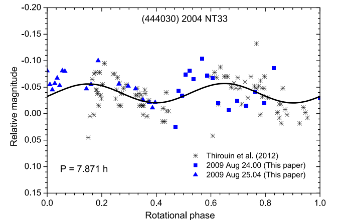
Figure 14. Double-peaked composite light curve of (444030) 2004 NT33. Zero phase is at UT 2009 August 24.6685.
