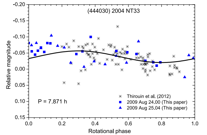
Figure 13. Single-peaked composite light curve of (444030) 2004 NT33. Zero phase is at UT 2009 August 24.6685.
