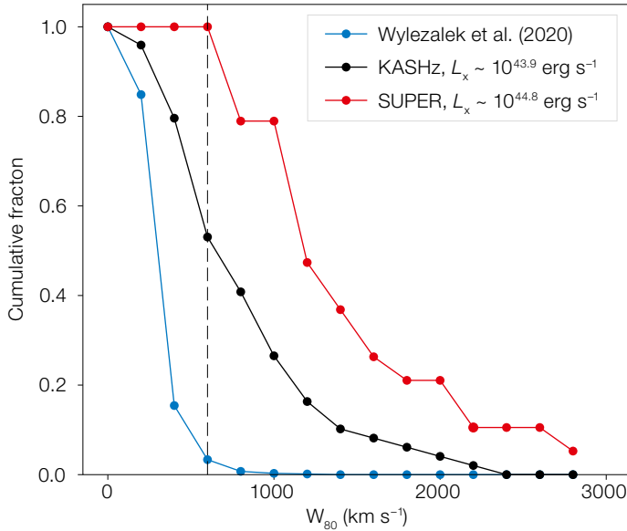
Figure 3. The inverse cumulative W80 distribution for the Type-1 AGN in the SUPER survey (red; Kakkad et al., 2020), the KASHz survey matched in redshift (black; Harrison et al., 2016), a mass-matched low-redshift star-forming sample (blue; Wylezalek et al., 2020). The dashed black-line at 600 km s -1 corresponds to the W80 value used to define that a target hosts an AGN-driven outflow (well justified from the fact that almost all star-forming galaxies have W80 values below this cut). Based on the above W80 criteria, all the Type-1 targets in SUPER show the presence of outflows, and ~ 52% of the redshift matched targets in the KASHz survey show outflows. The difference between the W80 distributions for SUPER and KASHz surveys is due to the different luminosity range of the AGN sampled by these surveys.
