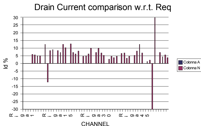
Figure 1 Current consumption of LFI from CRYO-02 respect to average ILT results. Values are expressed in percentage of Id. The hard requirement is \pm 5\% . Channel RCA 18 main is here different w.r.t. ILT because it was substituted with the Flight Spare after a failure occurred at phase switch level.
