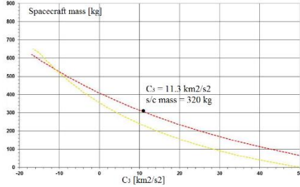
Fig. 7. Performance of Vega (launch mass, kg) with the PM endowed with either of two versions of the propellant tank (long in red, short in yellow).
