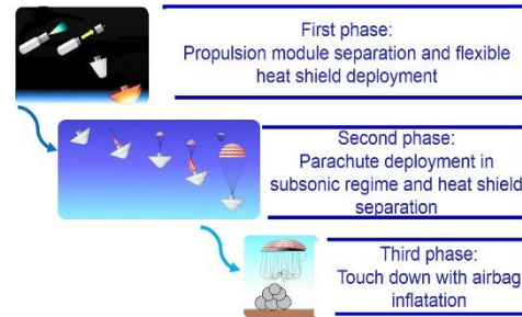
Figure 3. EDL operation sequence.
