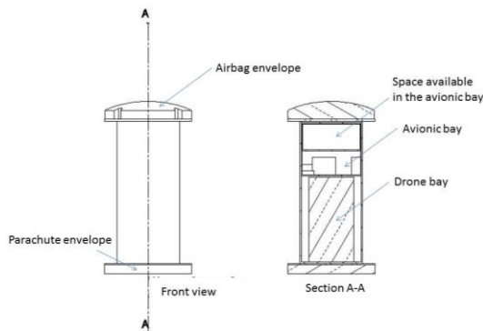
Fig. 2. SMS capsule configuration.
