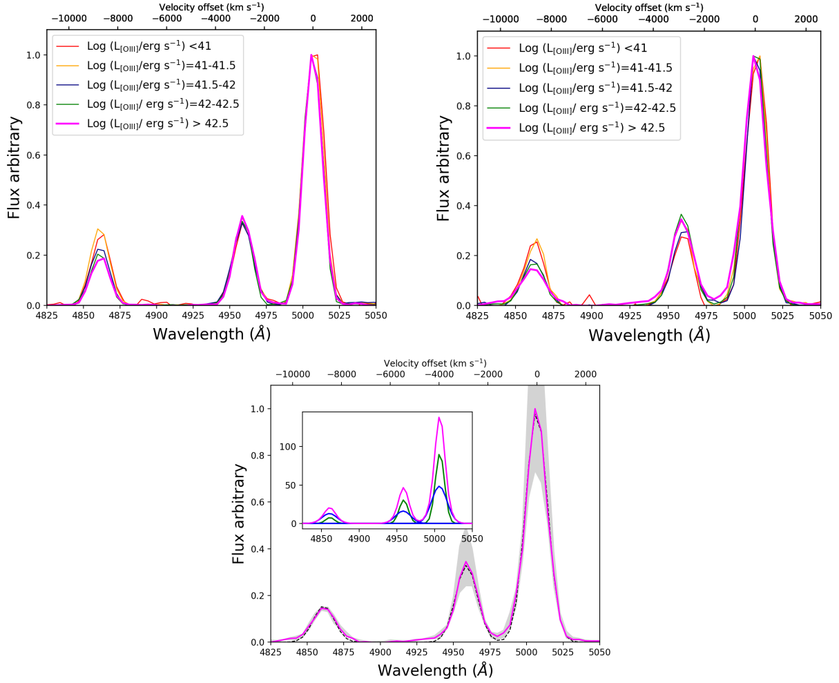
Fig. 7. Comparison of the stacked spectra, in the H \beta –[OIII] doublet lines wavelength range, in bins of [OIII] \lambda 5007 luminosity above ( left ) and below ( right ) the line threshold, as defined in Sect. 4.2 ( lower panel ). Stacked spectrum in the [OIII] luminosity bin \text{Log}(L_{[\text{OIII}]}/\text{erg s}^{-1}) > 42.5 of the low-SF Type II AGN with superimposed the 1\sigma uncertainties estimated through a bootstrap resampling technique and the best-fitting one-component Gaussian curve (black dashed line). The inset shows the best-fit double-Gaussian model (magenta curve) and its line decomposition (green and blue Gaussian profiles refer to the narrow and broad best-fit components).
