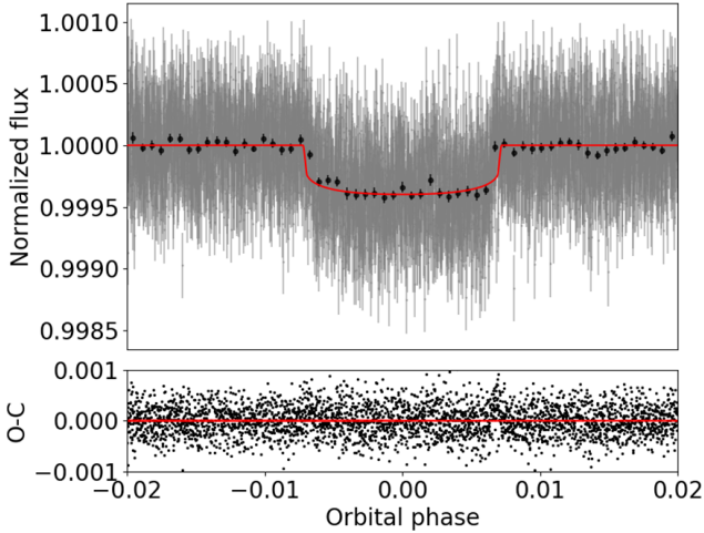
Fig. 6. Top : phase-folded transit light curve of HD 5278 b from eight individual transit events. The best-fit transit model produced in the combined ESPRESSO and TESS data analysis in Sect. 4.3 is depicted by the red curve. The black dots represent data averaged over 13.8 min bins. Bottom : post-fit residuals.
