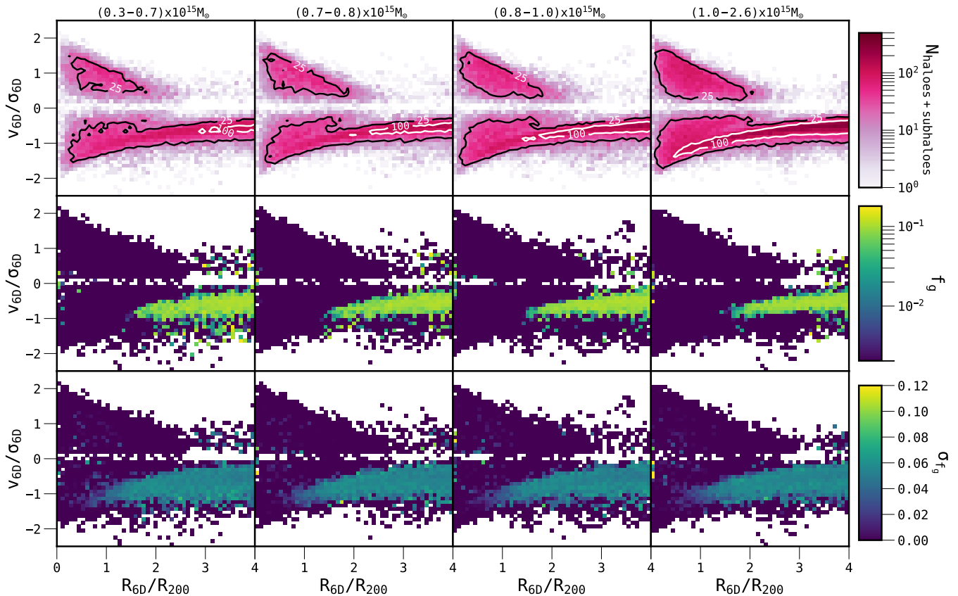
Figure 6. As in Fig. 5, but only shown for the 6D perspective and also binned by cluster mass. Each column represents one cluster mass bin, where the mass range is indicated above the top panel. The bin edges were chosen so that each bin contains 81 clusters. It is clear that as the cluster mass increases, the number of haloes and subhaloes on the plane also increase. The shape of the plane is not drastically different between bins. In all bins there is a sharp cut-off in the gas richness of infalling objects at \sim 1.5 R_{200} , which seems independent of cluster mass.
