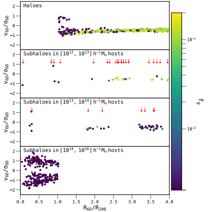
Figure 4. The phase-space plane for all haloes and subhaloes residing within 4 R_{200} of cluster 0005 (an example case) in the THE300 project. The top panel shows the phase-space information for the haloes in and around the cluster, whilst the bottom three panels show subhaloes; each panel is binned by the host mass that the subhaloes reside in, as indicated at the top-left of each panel. Each halo and subhalo are colour-coded by gas fraction. The red arrows in the bottom three panels mark the positions of the host haloes that the subhaloes reside in. In this example subhaloes are more gas-poor and their gas fractions decrease as the host halo's mass increases.
