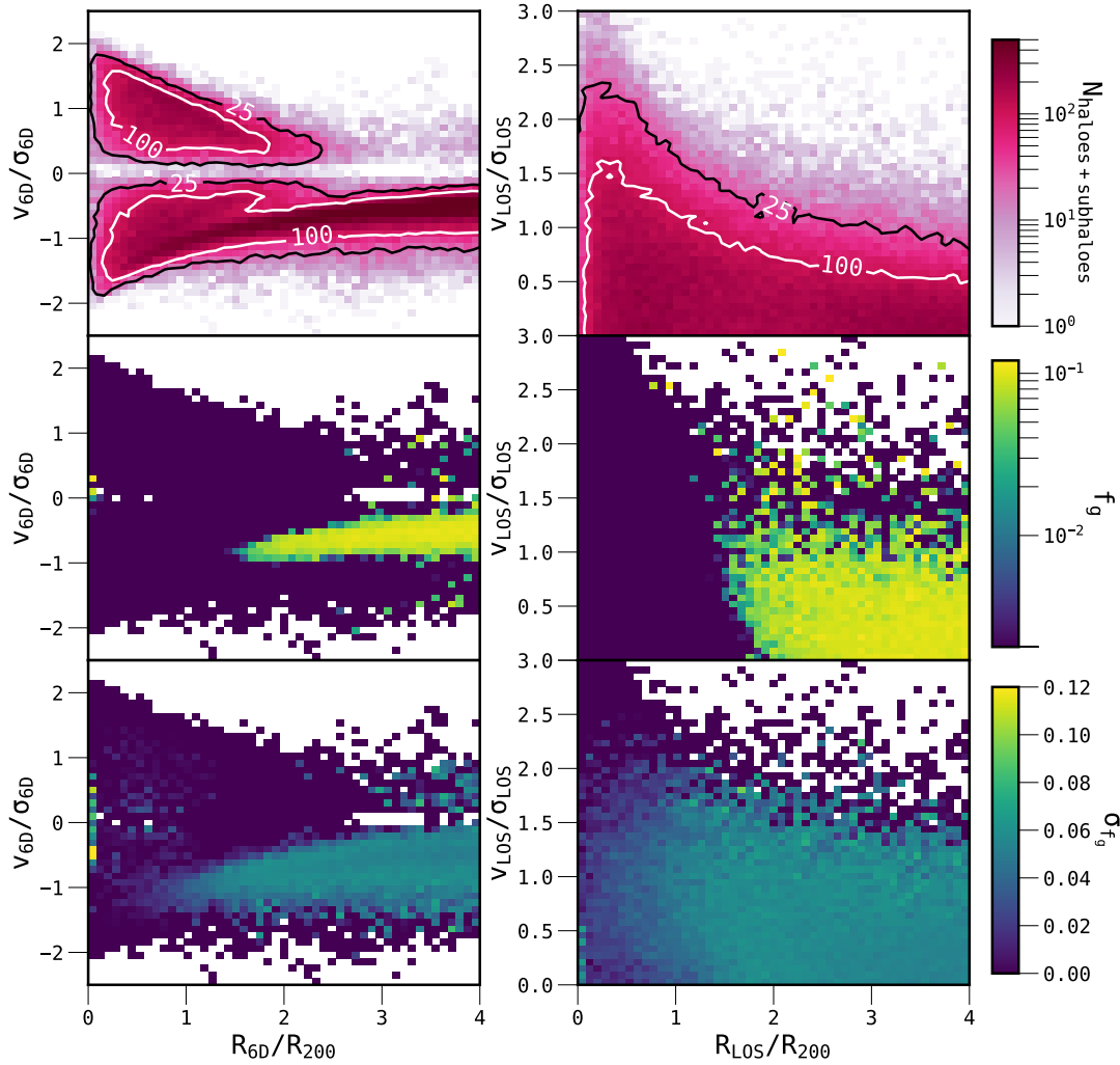
Figure 5. The stacked phase-space plane for all 324 clusters in the THE THREE HUNDRED project. Both haloes and subhaloes are included in all panels. The left and right columns are in 6D and LOS perspectives respectively. The planes are stacked on a 50 \times 50 grid where the top row shows the number of haloes and subhaloes in each bin, the middle row indicates the median gas fraction in each bin and the bottom row illustrates the gas fraction standard deviation in each bin. Contours are included in the top row, indicating the number of haloes and subhaloes encapsulated in each. The 6D perspective shows two distinct infalling and outgoing populations of objects, which is not seen in the LOS perspective. Also, from the the 6D perspective, first infallers are substantially more gas-poor and appear to lose their gas at \sim 1.5 R_{200} , whereas the cut-off in gas rich objects in the LOS perspective occurs closer to \sim 2 R_{200} .
