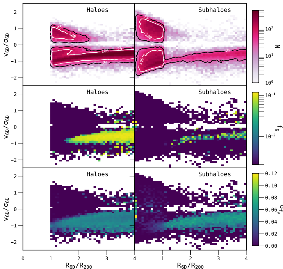
Figure 7. The stacked phase-space planes for all 324 clusters in the THE300 project, split by subhalo status. The left- and right-hand columns show only haloes and subhaloes respectively in the 6D perspective. The planes are constructed like in Fig. 5. \sim 10 percent of all infalling objects are in the form of subhaloes, which are substantially more gas-poor than haloes in the same phase-space location.
