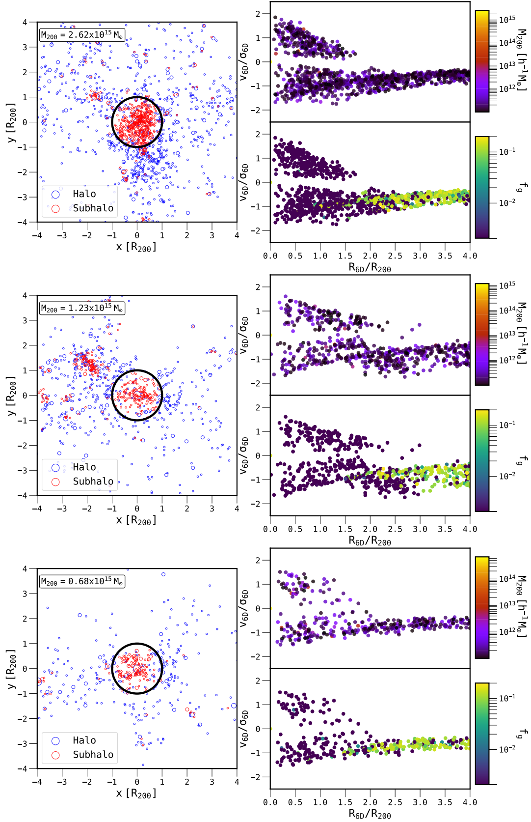
Figure 3. Three sample cluster resimulations from the THE300 project are shown. For each resimulation, the left panel shows the projected halo and subhalo spatial distributions in blue and red respectively. The black circle indicates where R_{200} of the cluster in the centre is. In the right panels, the 6D phase-space information for all of these haloes and subhaloes can be found. The top and bottom phase-space panel for each region are colour-coded by M_{200} and gas fraction respectively. THE300 project enables access to this information in a range of cluster environments, and it is apparent in these examples that the halo and subhalo gas fraction may be correlated with phase-space location.
