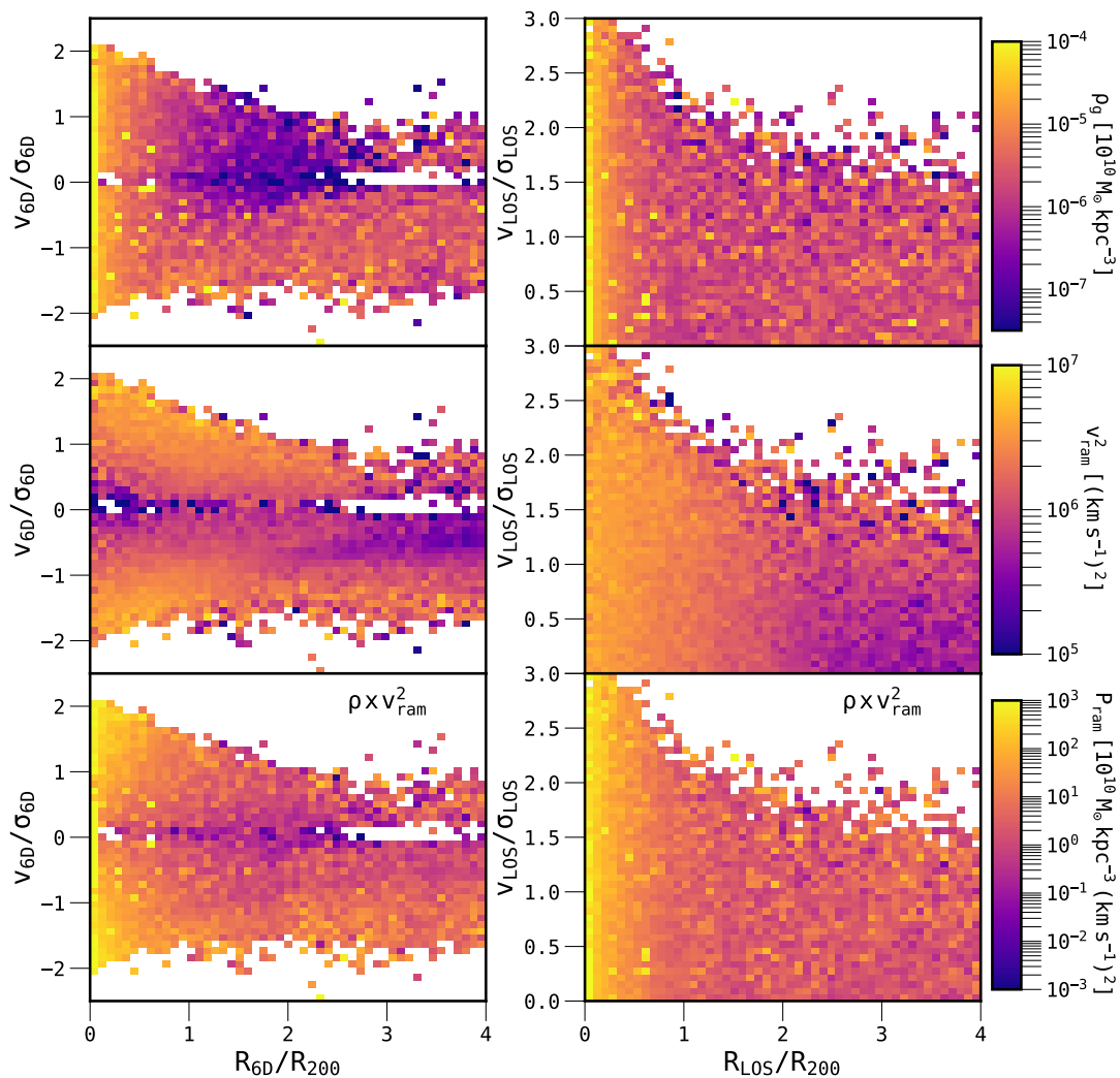
Figure 9. The stacked phase-space planes for all 324 clusters in the THE300 project, including both haloes and subhaloes. Here, the panels depict the effects of each term in Eq. 4, used for calculating the instantaneous ram pressure. The planes are stacked on a 50 \times 50 grid where the top row is colour-coded by the median local gas density in each bin, the middle row is colour-coded by the median differential velocity between the objects in each bin and their local gas, and the bottom row is colour-coded by the product of the first two rows as calculated by using the method described in Section 2.5. The left and right columns show the 6D and LOS perspectives, respectively. The 6D perspective shows that infalling objects typically experience higher local gas density than the outgoing population, but this is washed out in the LOS perspective. There are distinct regions in the phase-space planes with low v_{\text{ram}}^2 , and these line up well with the regions of high object gas fractions in Fig. 5.
