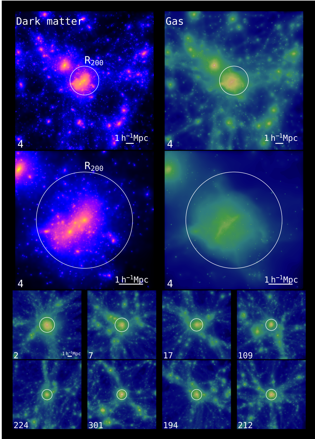
Figure 1. The figure shows nine example clusters from the THETHREEHUNDRED project at z = 0 . The top four panels are common to the same cluster, whilst the bottom eight panels each show a different cluster. The number in the bottom-left of each panel corresponds to the cluster number in the THETHREEHUNDRED database. For cluster 4, the left and right panels show the projected dark matter and gas distributions respectively. For all other clusters, only the projected gas distribution is shown. Two perspectives are shown for cluster 4. The top panels show a 20 h^{-1} \text{Mpc} \times 20 h^{-1} \text{Mpc} view of the simulation (this projection is also used for the clusters in the bottom eight panels), whilst the bottom panels show a 6 h^{-1} \text{Mpc} \times 6 h^{-1} \text{Mpc} view. The white circle in each panel represents where R_{200} is for each cluster halo. The figure demonstrates the suitability of the data for this study, as it contains a statistically significant sample of massive clusters embedded in a wide range of environments, a full treatment of the gas and a large resimulation volume that includes many filamentary and group structures around each cluster.
