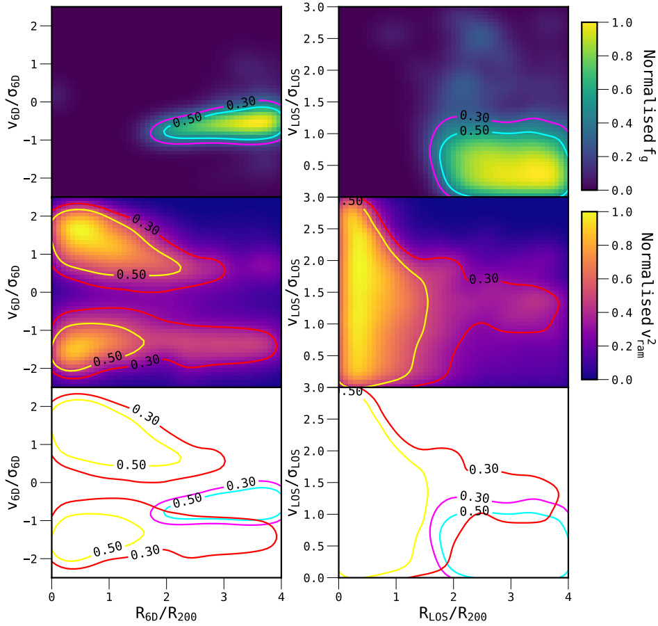
Figure 10. In both the 6D and LOS perspectives, the figure shows the middle-row panels from Fig. 5 (top row) and Fig. 9 (middle row). Here though, the planes have been convolved with a gaussian and then normalised. The bottom row illustrates how the contours from each plane align. Though there is some overlap, the contours from f_g and v_{\text{ram}}^2 appear almost mutually exclusive with each other.
