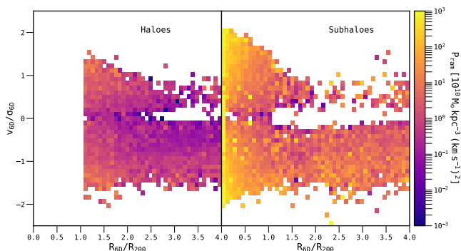
Figure 12. As in Fig. 7, but coloured according to the median instantaneous ram pressure on haloes and subhaloes in each bin. Subhaloes experience around two orders of magnitude more ram pressure than their halo counterparts in any region of the phase-space plane.
