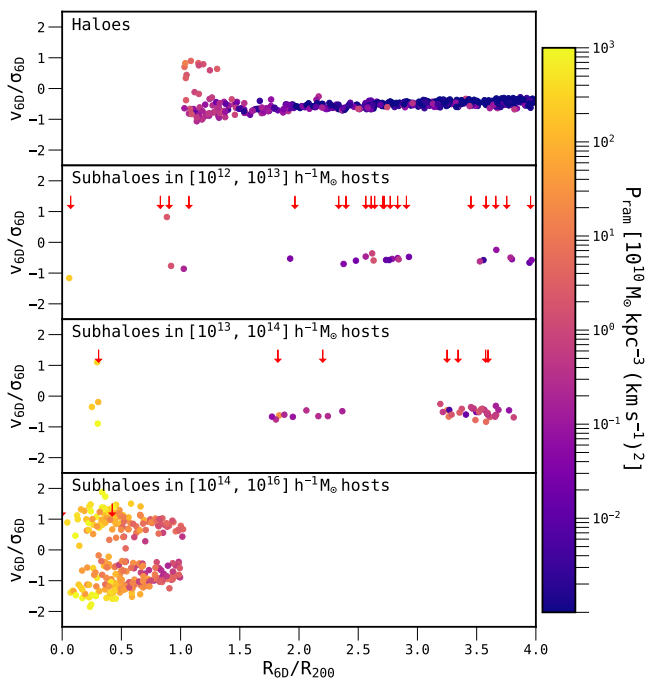
Figure 8. As in Fig. 4, but each halo and subhalo are now colour-coded by instantaneous ram pressure, calculated using the method described in Section 2.5. The red arrows in the bottom three panels mark the positions of the host haloes that the subhaloes reside in. The figure demonstrates how we can use the wealth of information provided by THETHREEHUNDRED to investigate how the instantaneous ram pressure correlates with phase-space position, cluster environment and subhalo status. In this example, subhaloes are experiencing more ram pressure compared to haloes at the same phase-space location and this seems to be proportional with their host mass.
