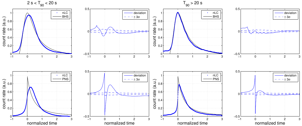
Figure 6. Phase III matched filtering analysis of BATSE against the model light curve of Fig. 4 (top panels) and that of a proto-neutron star (lower panels). Consistency is relatively better for the former, especially so for durations greater than 20 s. We attribute this time-scale to that of jet breakout of a stellar remnant envelope. (Adapted from van Putten 2012.)
