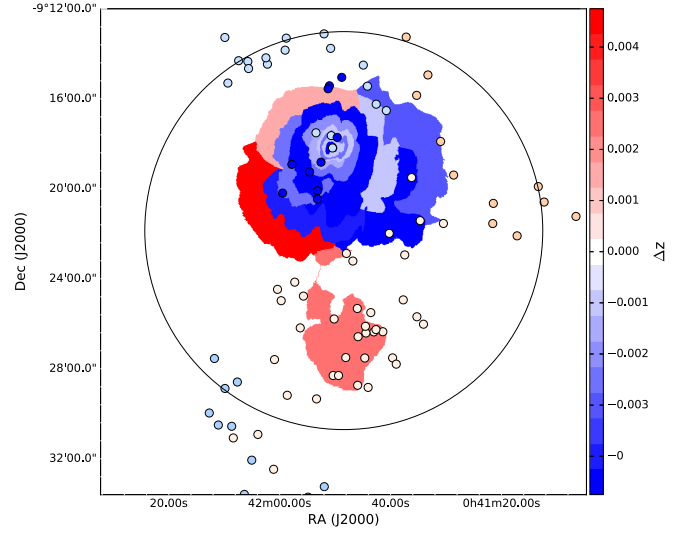
Figure 9. Redshift deviation map of the ICM of A85 with respect to its average redshift ( z_{\text{avg}} = 0.0554 ). The bin size of the colored bar is \delta z = 0.001 . The galaxies (circles) are colored with the same redshift scale.
