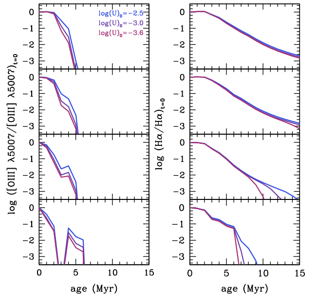
Figure 5. Evolution of the line luminosity relative to the initial one at t = 0 for [O III] (left) and H \alpha (right) as a function of time, metallicity and \log(U)_0 . Metallicity ( Z = 0.004, 0.008, 0.02 and 0.04 ) increases from the top to the bottom panel. In each panel, we show the results for \log(U)_0 = -2.5, -3 and -3.6 , with \log(U)_0 decreasing from blue to red, as indicated.
