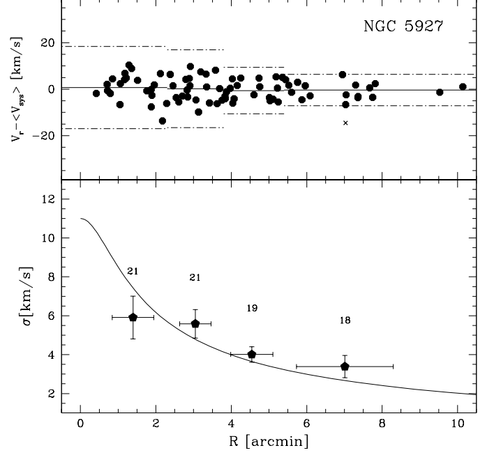
Fig. 15. Same as in Fig. 9, but for NGC 5927. Core radius ( r_C = 1.40' ) and concentration ( C = 1.60 ) are from Trager et al. (1993) and K66 models are normalised to \sigma_0 = 11.0 \text{ km s}^{-1} (continuous line; our estimate).
