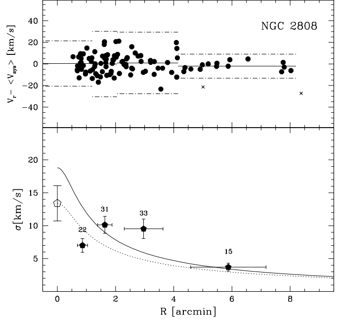
Fig. 12. Same as in Fig. 9, but for NGC 2808. Core radius ( r_c = 0.26' ) and concentration ( C = 1.8 ) are from Trager et al. (1993) and K66 models are normalised to \sigma_0 = 18.8 \text{ km s}^{-1} (continuous line; our estimate) and \sigma_0 = 13.4 \text{ km s}^{-1} (dotted line; by Pryor & Meylan 1993). The open pentagon is the value of \sigma at the centre from Pryor & Meylan (1993).
