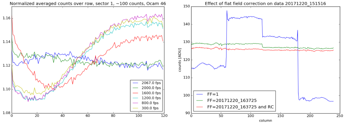
(a) Average counts on the rows with uniform illumination ( \sim 100 counts) over half the 120 \times 120 central sub-frame. The values are normalized by the average on the sector. Different colors represent different frame rates. (b) Average counts over the rows for the sectors in the bottom part of the chip (from 0 to 3). Blue line is wit no flat fielding, green line flat fielding with a previous power cycle and red line is flat fielding from a previous power cycle with the sector by sector re-normalization.
