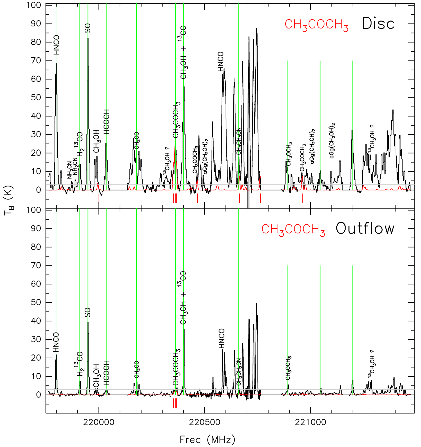
Figure A14. Synthetic spectra for \text{CH}_3\text{COCH}_3 overplotted on the observed spectrum for the disc and outflow positions as in Fig. 1. The red line corresponds to the synthetic spectrum fitted using xCLASS and the vertical red lines indicate the detected transitions above 5\sigma for this particular species. Vertical green lines mark the transitions whose zeroth-order moment has been imaged and is shown in Figs 2 and 3. The grey horizontal line marks the 5\sigma detection threshold.
