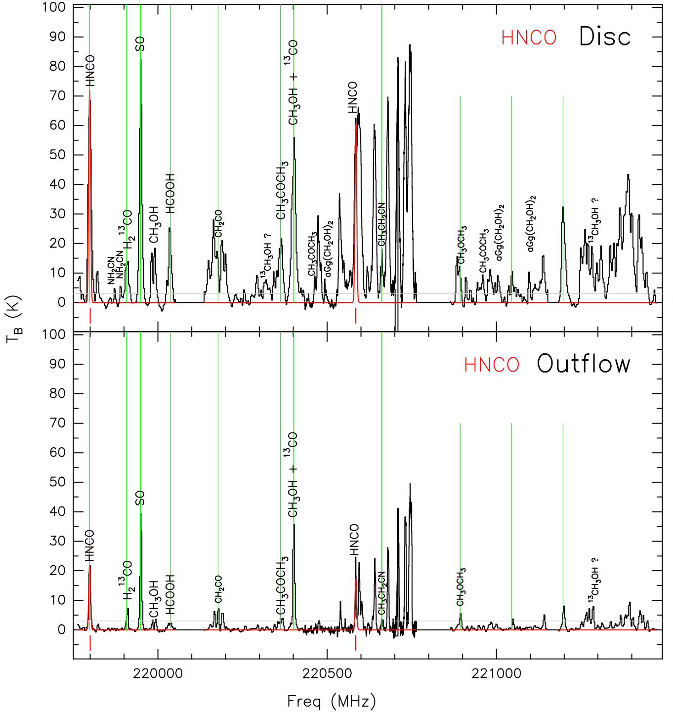
Figure A4. Synthetic spectra for HNCO overplotted on the observed spectrum for the disc and outflow positions as in Fig. 1. The red line corresponds to the synthetic spectrum fitted using xCLASS and the vertical red lines indicate the detected transitions above 5\sigma for this particular species. Vertical green lines mark the transitions whose zeroth-order moment has been imaged and is shown in Figs 2 and 3. The grey horizontal line marks the 5\sigma detection threshold.
