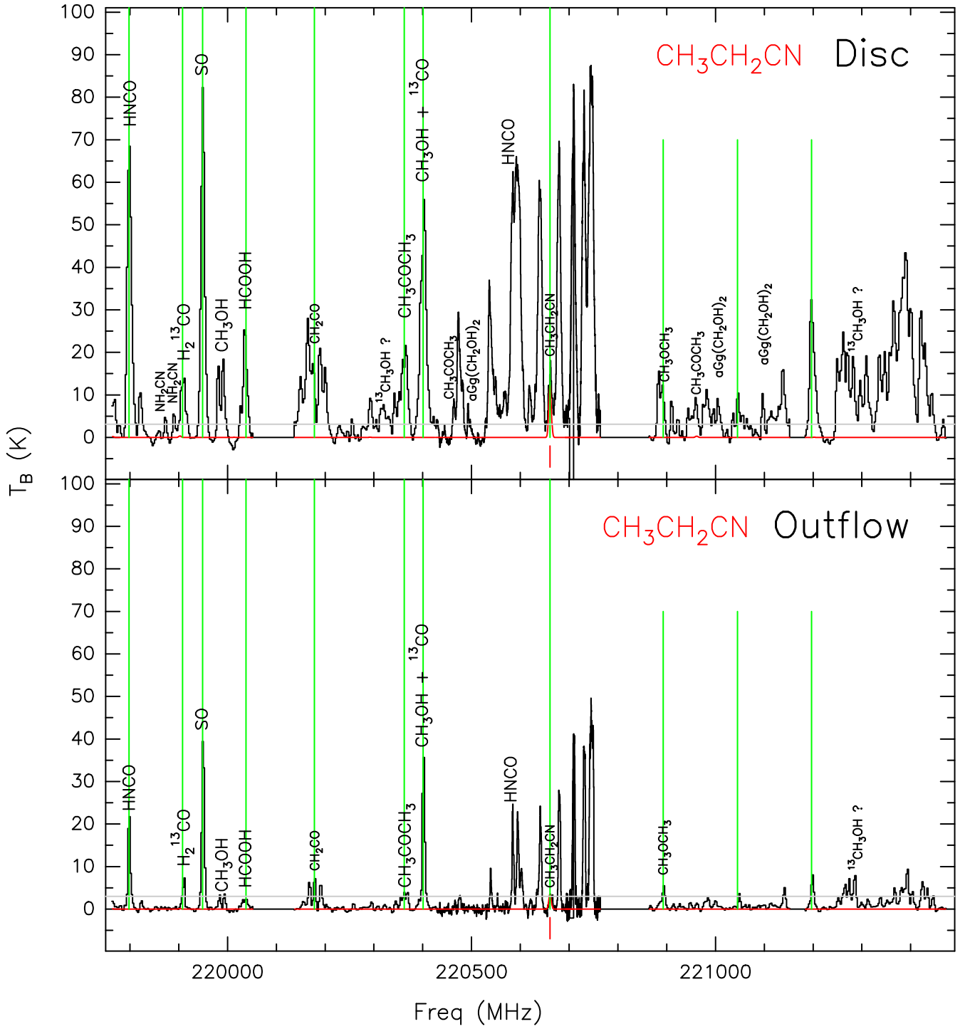
Figure A12. Synthetic spectra for \text{CH}_3\text{CH}_2\text{CN} overplotted on the observed spectrum for the disc and outflow positions as in Fig. 1. The red line corresponds to the synthetic spectrum fitted using xCLASS and the vertical red lines indicate the detected transitions above 5\sigma for this particular species. Vertical green lines mark the transitions whose zeroth-order moment has been imaged and is shown in Figs 2 and 3. The grey horizontal line marks the 5\sigma detection threshold.
