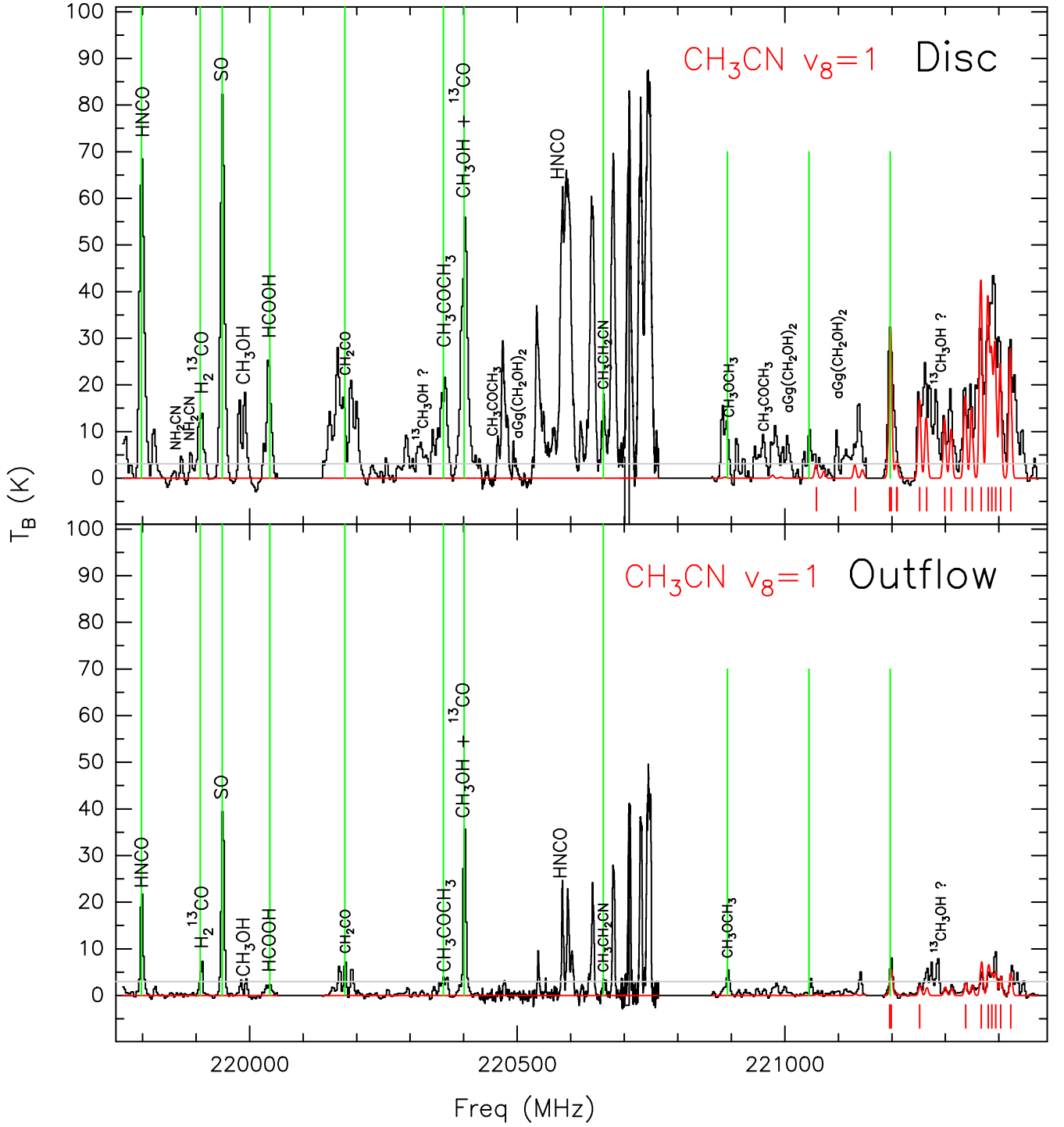
Figure A10. Synthetic spectra for \text{CH}_3\text{CN}-v_8 = 1 overplotted on the observed spectrum for the disc and outflow positions as in Fig. 1. The red line corresponds to the synthetic spectrum fitted using xCLASS and the vertical red lines indicate the detected transitions above 5\sigma for this particular species. Vertical green lines mark the transitions whose zeroth-order moment has been imaged and is shown in Figs 2 and 3. The grey horizontal line marks the 5\sigma detection threshold.
