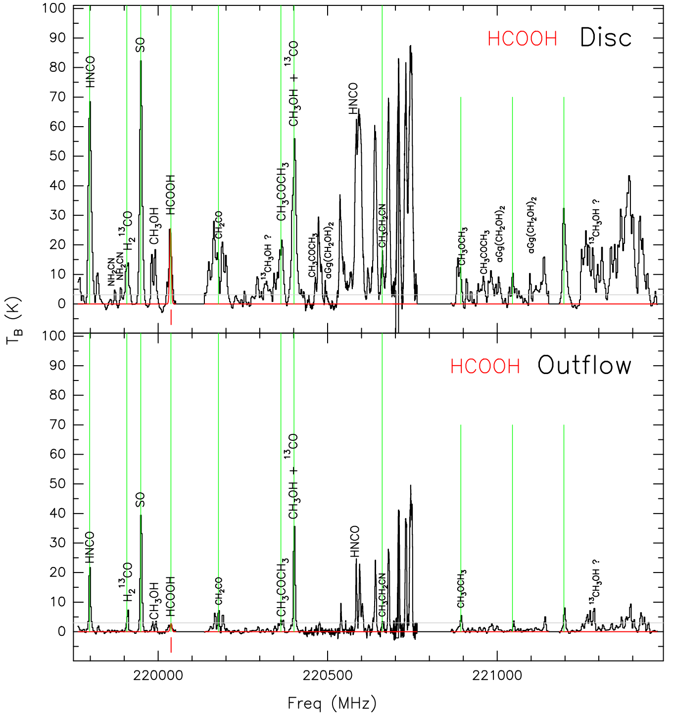
Figure A6. Synthetic spectra for HCOOH overplotted on the observed spectrum for the disc and outflow positions as in Fig. 1. The red line corresponds to the synthetic spectrum fitted using XCLASS and the vertical red lines indicate the detected transitions above 5\sigma for this particular species. Vertical green lines mark the transitions whose zeroth-order moment has been imaged and is shown in Figs 2 and 3. The grey horizontal line marks the 5\sigma detection threshold.
