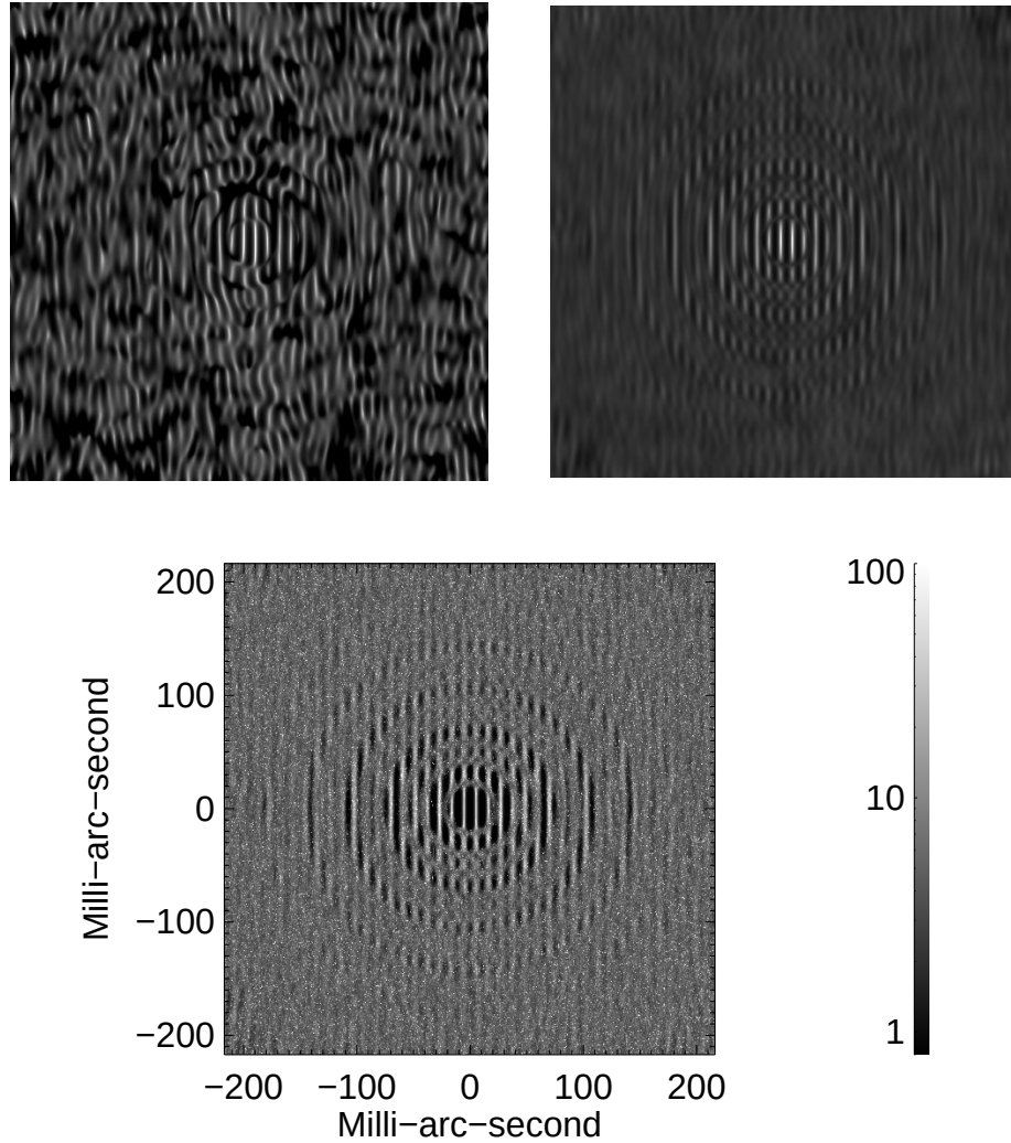
Figure 5. Contrast gain map of the LBTI vs the LBT. Ratio of a short exposure (top left), ratio of the long exposure G_{LE} (top right) and average of the ratio of the short exposures G_{SE} (bottom). Logarithmic scale.
