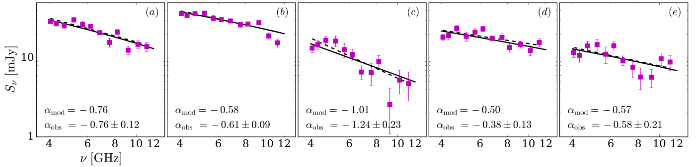
Fig. 5. Observed flux densities (magenta squares) and their best fits (dashed black lines) for five positions in DS as function of frequency (panels a–e; see Fig. 5 in Meng et al. 2019). Solid black lines show the model results (see Table 1 for a complete overview of the model parameters). Each subplot also displays the modelled and observed spectral indexes, \alpha_{\text{mod}} and \alpha_{\text{obs}} , respectively.
