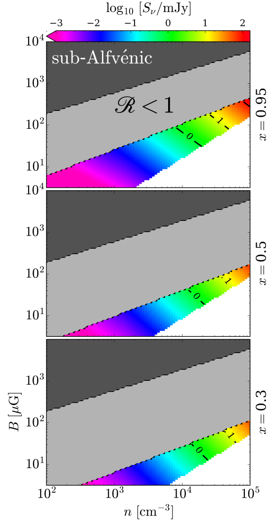
Fig. A.1. Flux density, S_\nu , for T = 7500 K, U = 40 km s ^{-1} , L = 0.5 pc, \nu = 300 MHz, and \theta_b = 10'' in parameter space ( n, B ) for three different values of ionisation fraction as labelled on right-hand side of each subplot. Dark and light grey-shaded areas in each subplot show the region of the parameter space where the condition of super-Alfvénic flow and ion-neutral coupling is not satisfied, respectively. Solid black lines in each subplot show the iso-flux density at 1 and 10 mJy in logarithmic scale (from the bottom up).
