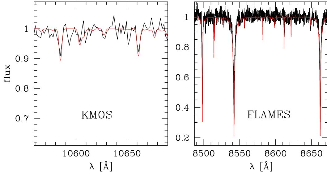
Fig. 1.— Examples of KMOS (left) and FLAMES (right) spectra. The observations are plotted in black, while the synthetic templates are in red. Fluxes are arbitrarily normalized to unit.
