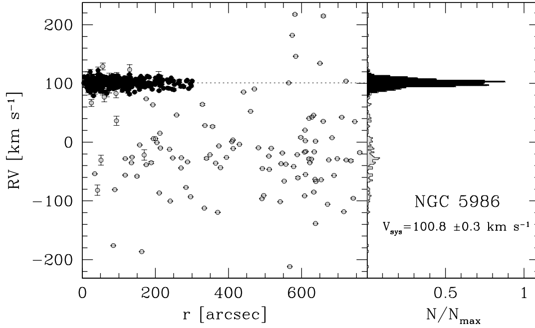
Fig. 2.— Left panel: Radial distribution of the line-of-sight velocities measured from the MIIIS observations in NGC 5986. The selected cluster members are plotted as black circles, while field contaminants are in grey. Right panel: RV distribution as a normalized histogram. V_{\text{sys}} denotes the cluster systemic velocity.
