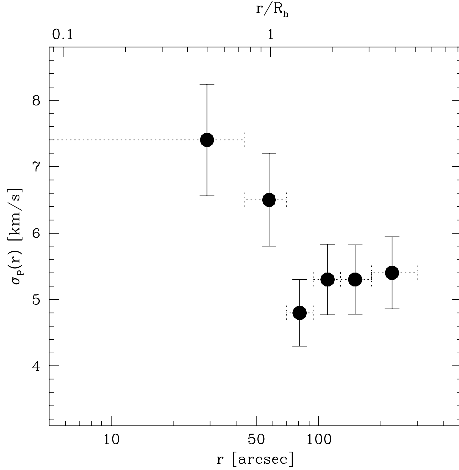
Fig. 7.— Projected velocity dispersion profile, determined after subtraction of the rotational contribution to the individual RVs, in six concentric annuli around the cluster center.
