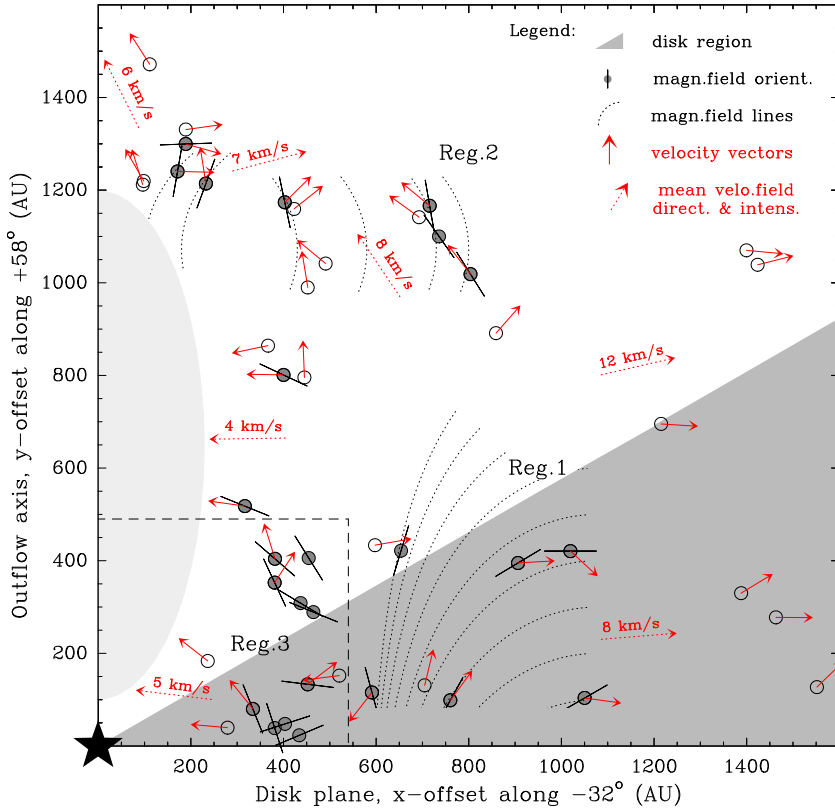
Fig. 4. Combined plot of the velocity and magnetic field measurements obtained from the 6.7 GHz \text{CH}_3\text{OH} maser cloudlets (dots) in G023.01–00.41. The axes are aligned with the outflow and disk directions, as defined by the subarcsecond SMA observations in the 1 mm band from Sanna et al. (2014). The origin is set at the HMC center, as defined in Sect. 3 (star symbol in Fig. 2). The dark gray area indicates the region where emission from a flared disk with axes ratio of 1/2 is expected. The light gray area shows the region close to the outflow axis that is devoid of maser emission. For each maser cloudlet, the local directions of the velocity vector (red solid arrows) and/or that of the magnetic field vector (black solid lines) are reported where available. Empty dots are used for cloudlets that do not show polarized emission. The local average of both the magnitude and direction of the velocity field is indicated by red dotted arrows. These values were derived by grouping close-by features with similar velocity directions. The different regions identified through the polarization vectors analysis (Fig. 3) and labeled from 1 to 3 are indicated. For regions showing a smooth variation in the polarization (and magnetic) field vectors with the maser cloudlet position, we plot the families of curves (black dotted lines) that match the tangent to the local magnetic field measurements best (see Sect. 4). The pattern of these families of curves approximates the spatial morphology of the magnetic field lines locally. The direction of the velocity vectors is on average tilted by 30^\circ with respect to the local magnetic field direction.
