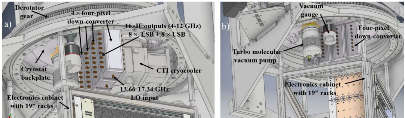
FIGURE 23. 3D sketches (left “a”, and right, “b”) showing the four independent four-pixel down-converter modules attached to the cryostat backplate. The backplate hosts the vacuum valve (not shown), the turbomolecular vacuum pump, the vacuum gauge, the CTI cryocooler, the WR10 waveguide vacuum feedthroughs and the vacuum feedthrough DC connectors for biasing the internal components of the cryostat.
