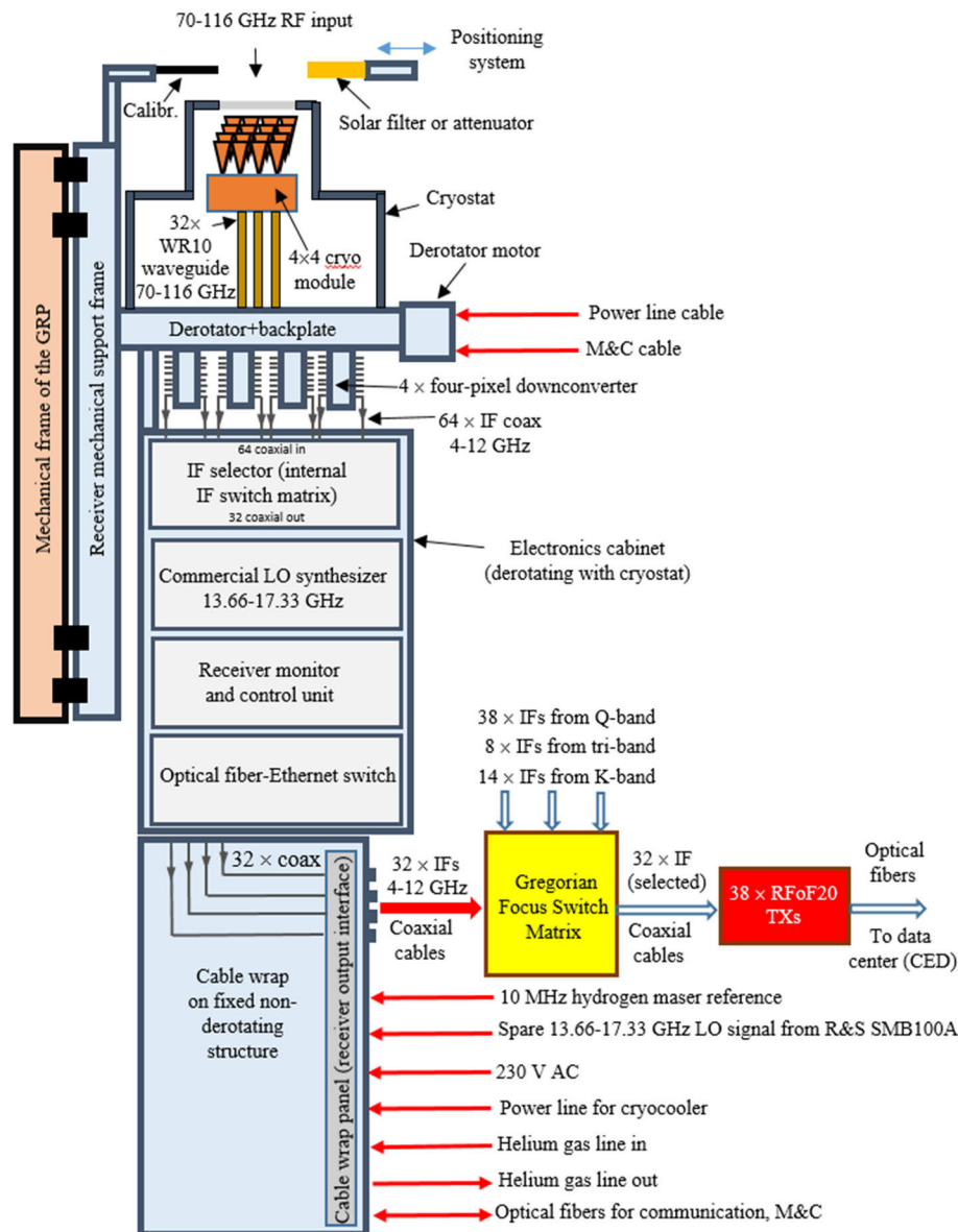
FIGURE 6. Schematic diagram of 70-116 GHz multibeam receiver (see also Fig. 4) showing the positioning system with calibrator and solar filter-attenuator, the cryostat with internal 4 \times 4 cryogenic array, the four four-pixel downconverters attached to the cryostat backplate at room temperature, the derotator, the electronics cabinet (with IF selector, LO synthesizer, M&C unit and optical fiber-Ethernet switch), the cable wrap, the receiver mechanical support frame bolted to the GRP mechanical frame. This schematic illustrates the interfaces between the receiver and the infrastructure available at the SRT. The red arrows indicate the connections that will be available at the receiver cable wrap panel, which includes the interfaces for: a) 32 coaxial cables with the 4-12 GHz IF output signals (to connect to the Gregorian focus switch matrix cascaded with the 38 RFoF20 optical transmitters); b) the 10 MHz hydrogen maser reference for phase-lock of the Local Oscillator; c) the spare 13.66-17.33 GHz baseband LO signal; d) the power line for the cryocooler; e) the Helium gas supply and return lines for the cryocooler; f) the single-mode optical fibers (Tx/Rx) for the receiver M&C. The derotator motor utilizes power line and M&C cables external to the cable wrap.
