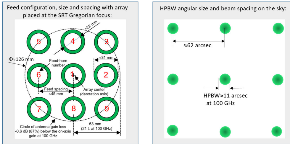
FIGURE 25. Left: Configuration of a 3 \times 3 array on the SRT Gregorian focal plane with 45 mm spacing between contiguous feeds. The diameter of the feed aperture is about 22 mm. Right: Sketch of 3 \times 3 beams projected on the sky showing the angular separation between contiguous beams (62 arcsec) and the HPBW \approx 11 arcsec of each beam at 100 GHz. The plate scale factor on the focal plane is 1.4 arcsec/mm. The example refers to an array of feeds placed on the Gregorian focus without re-imaging optics.
