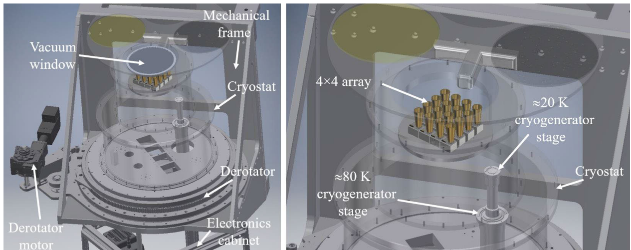
FIGURE 20. 3D sketch of the inner part of the cryostat showing the 4 \times 4 cryogenic array and the CTI cryogenerator (cold finger). Left panel: the vacuum window is located in front of the feed-horn cluster. Right panel: view of the 4 \times 4 array.
