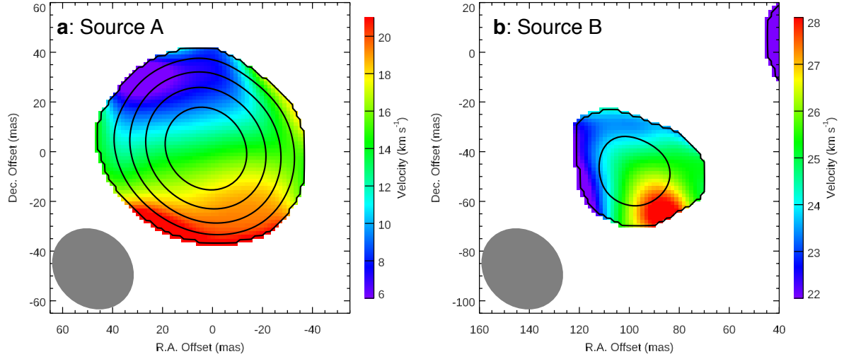
Supplementary Figure 2: The moment maps of the \text{H}30\alpha emission in Source A (panel a) and B (panel b). The moment 0 maps (integrated emission) are shown in the black contours and the moment 1 maps (intensity-weighted mean velocities) are shown in the color scale. The moment 0 map in panel a is integrated in the velocity range of -30 \text{ km s}^{-1} < V_{\text{lsr}} < 55 \text{ km s}^{-1} , and the contour levels are 5\sigma \times 2^n ( n = 1, 2, 3, \dots ) with 1\sigma = 13 \text{ mJy beam}^{-1} \text{ km s}^{-1} . The moment 0 map in panel b is integrated in the velocity range of -10 \text{ km s}^{-1} < V_{\text{lsr}} < 60 \text{ km s}^{-1} , and the contour levels are 5\sigma \times 2^n ( n = 1, 2, 3, \dots ) with 1\sigma = 14 \text{ mJy beam}^{-1} \text{ km s}^{-1} . The synthesized beam is shown in the bottom-left corner.
