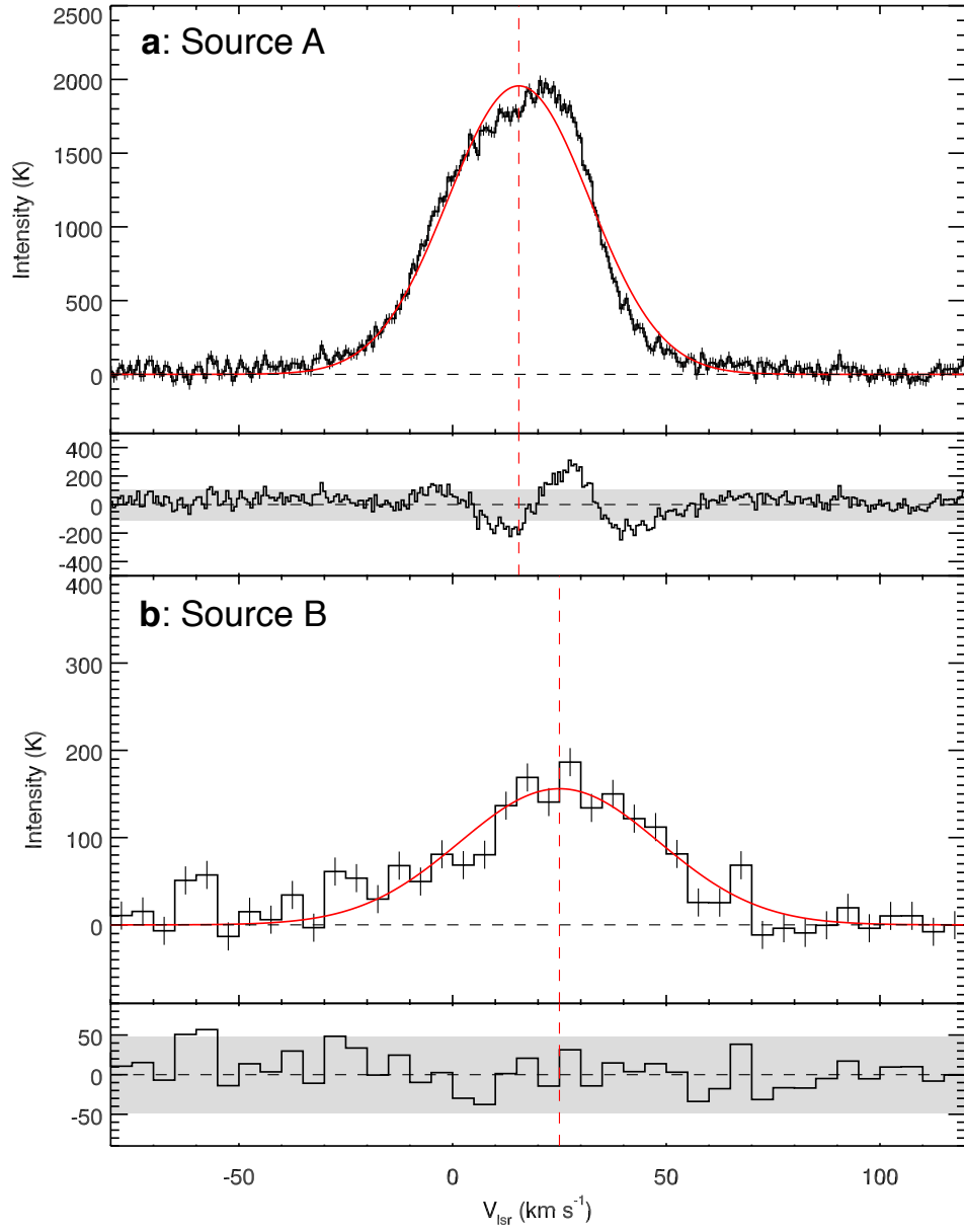
Figure 2: H30 \alpha line spectra at the continuum peak positions of Source A (panel a) and Source B (panel b). The r.m.s. noise levels are marked by the error bar in each velocity channel. The red solid curves are fitted Gaussian profiles with the central velocities indicated by the red dashed lines. The residual differences between the observed spectra and fitted Gaussian profiles are also shown below the spectra. The shaded regions indicate the 3\sigma noise levels.
