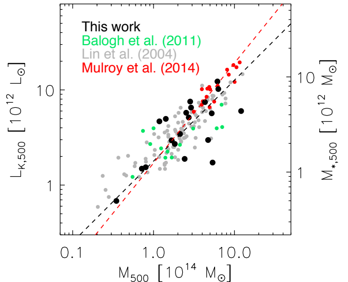
Fig. 7. M_{500} - L_{K,500} relation for this work and other works in the literature as indicated by the legend. The dashed lines show the best linear fit for XXL only (black) and XXL+LoCuSS (red). Balogh et al. (2011) and Lin, Mohr, & Stanford (2004) measure 3D luminosities, while we de-project L_K for XXL and LoCuSS (as in Mulroy et al., 2014) by multiplying these luminosities by 0.68 (see text for details).
