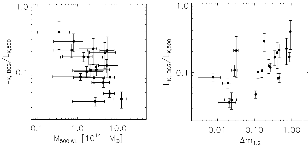
Fig. 6. Fractional contribution in luminosity of the BCG as a function of weak-lensing mass (left panel) and as a function of the magnitude gap between the two brightest members of the clusters (right panel).
