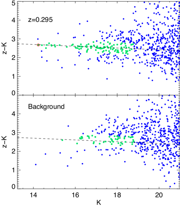
Fig. 1. Colour-magnitude diagram for all galaxies lying in the projected distance of r_{500,WL} for XLSSC 27 (at z = 0.295 ) in the XXL sample (top panel) and an area selected as background within the same projected distance (bottom panel). The dashed line shows the best linear fit for the candidate cluster members, also shown in the bottom panel for reference. The galaxies selected to account for the total K-band luminosity of the cluster and the field are shown in green ( K_{BCG} \leq K < K^* + 3 and \pm 0.3 mag from the dashed line), while the BCG is highlighted in red. The colour sequence for the clusters appears more populated (in particular at bright magnitudes) than the background region (field) as expected.
